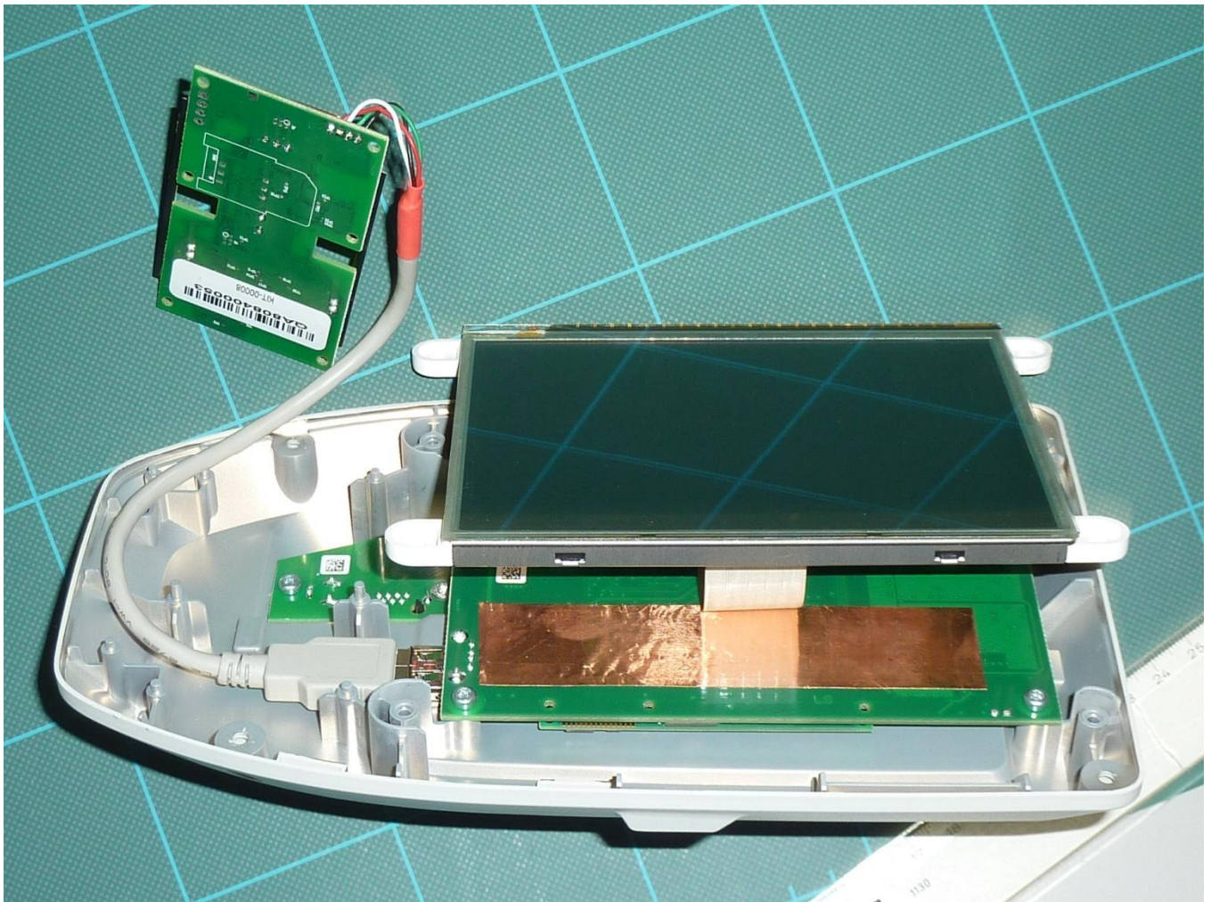
181775_eut10: Internal view 3
