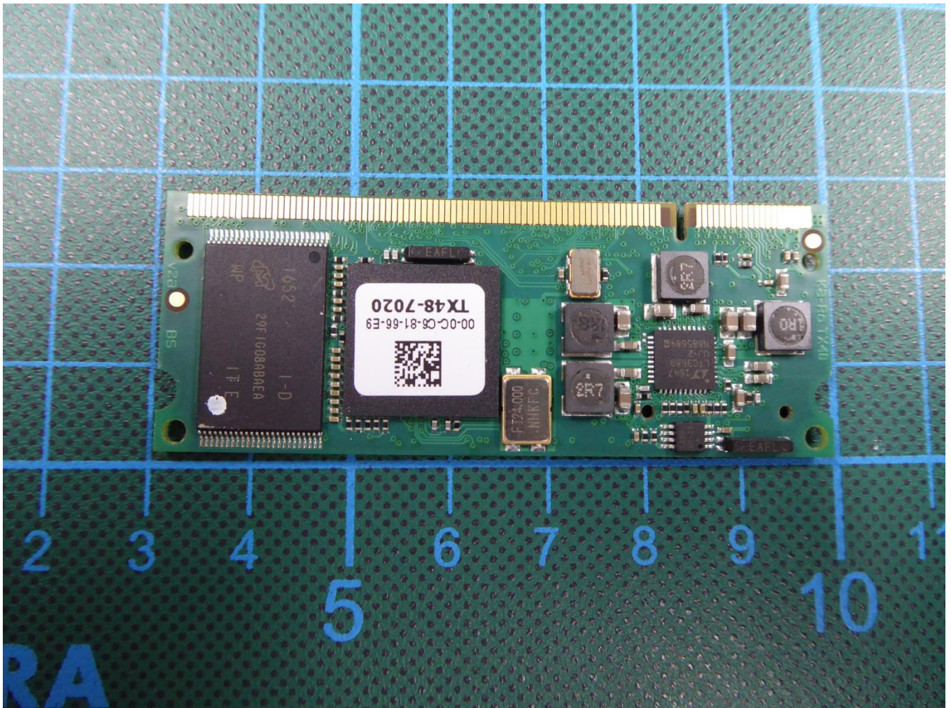
181775_eut16: Top view sub PCB
