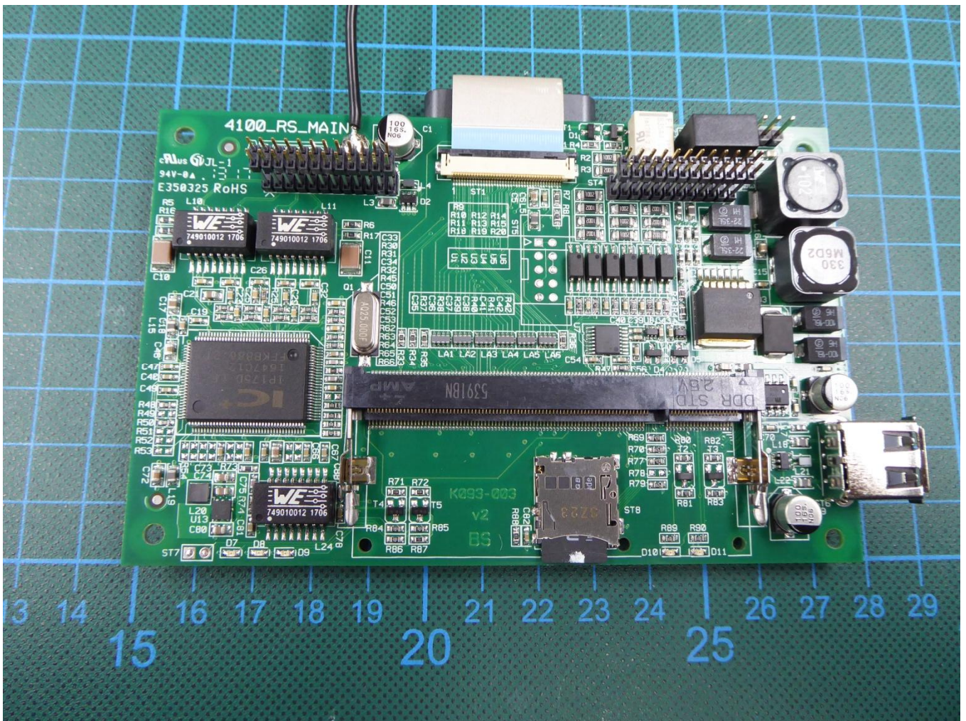
181775_eut15: Top view main PCB without sub PCB
