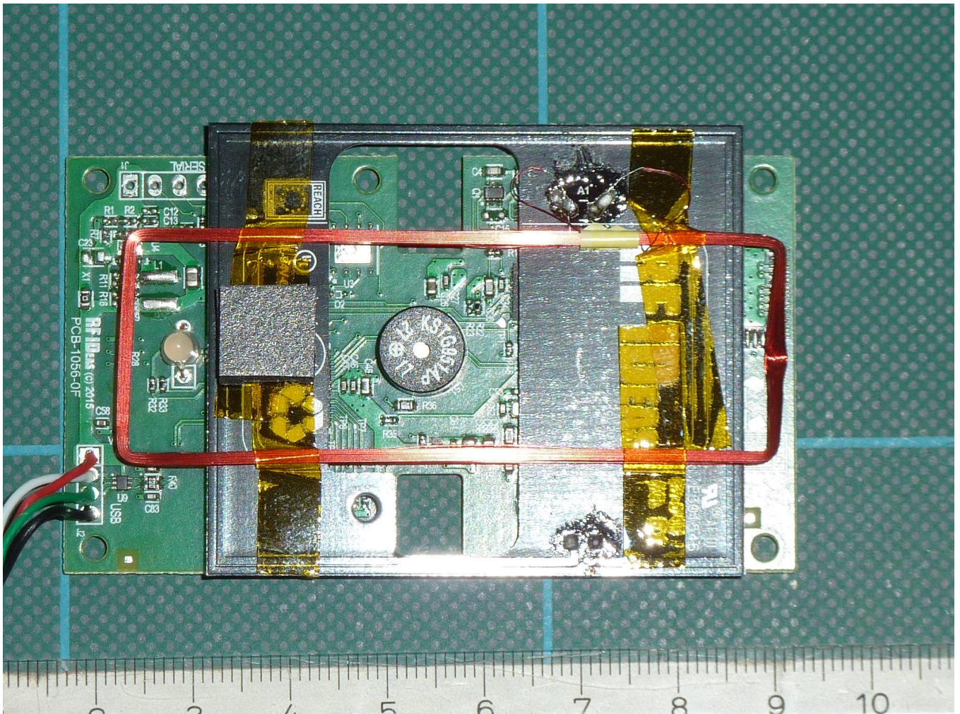
181775_eut23: Top view RFID PCB
