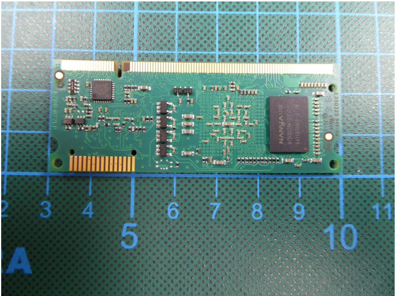
181775_eut17: Bottom view sub PCB
