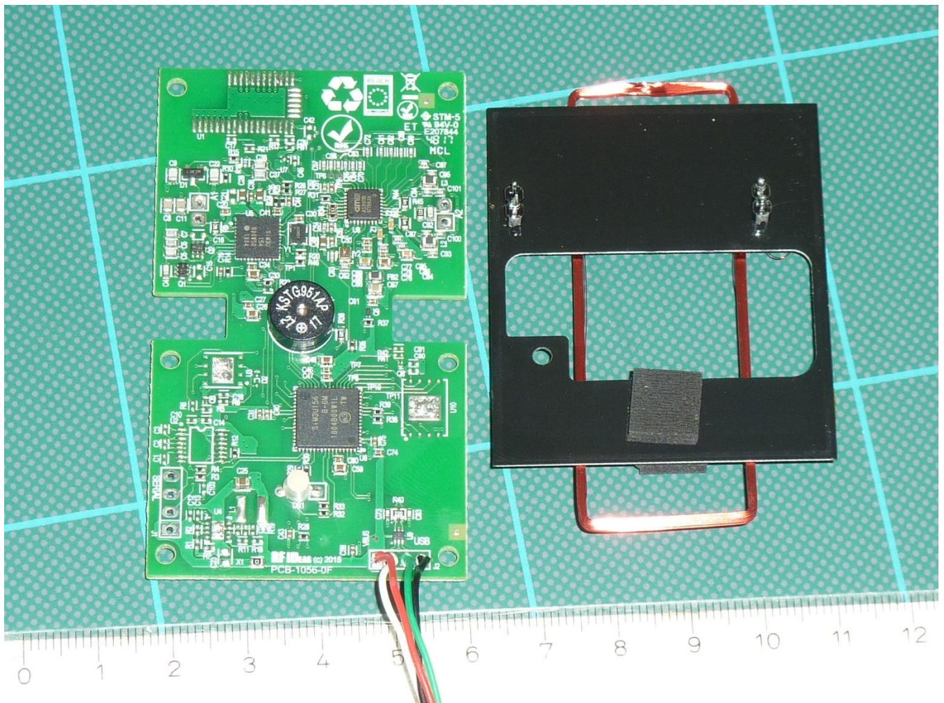
181775_eut24: View RFID PCB
