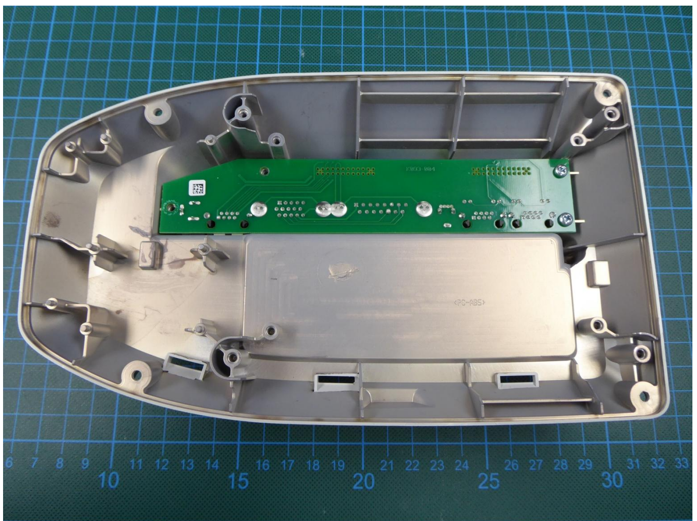
181775_eut18: Internal view 5
