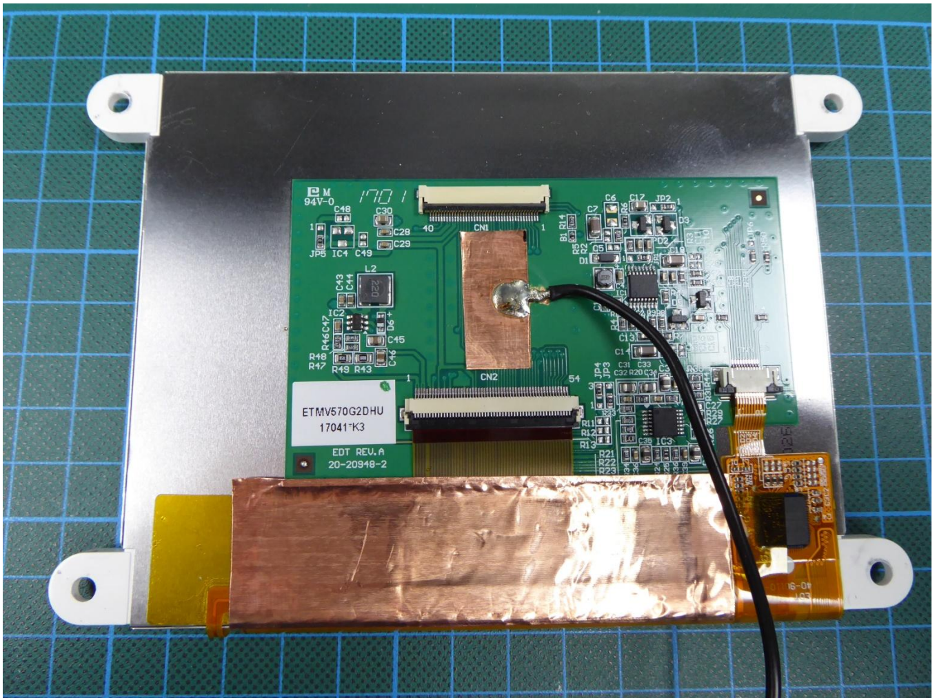
181775_eut13: Bottom view Display
