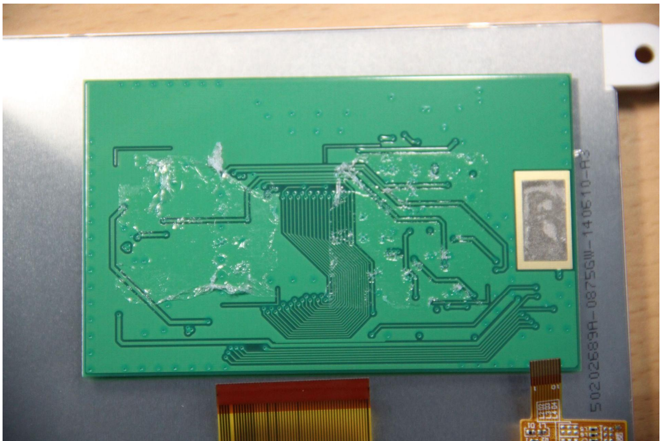
181775_eut13a: Bottom view PCB Display (this photo was delivered by the applicant)
