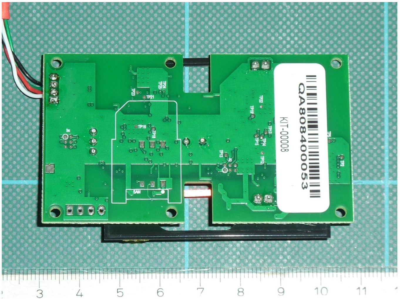
181775_eut22: Bottom view RFID PCB
