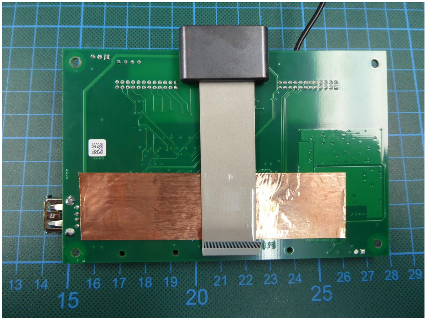
181775_eut12: Bottom view main PCB
