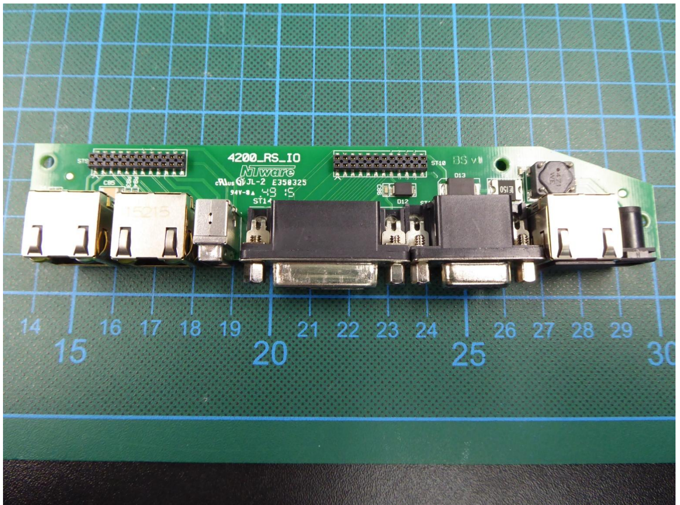
172189_eut21: Top view connector PCB
