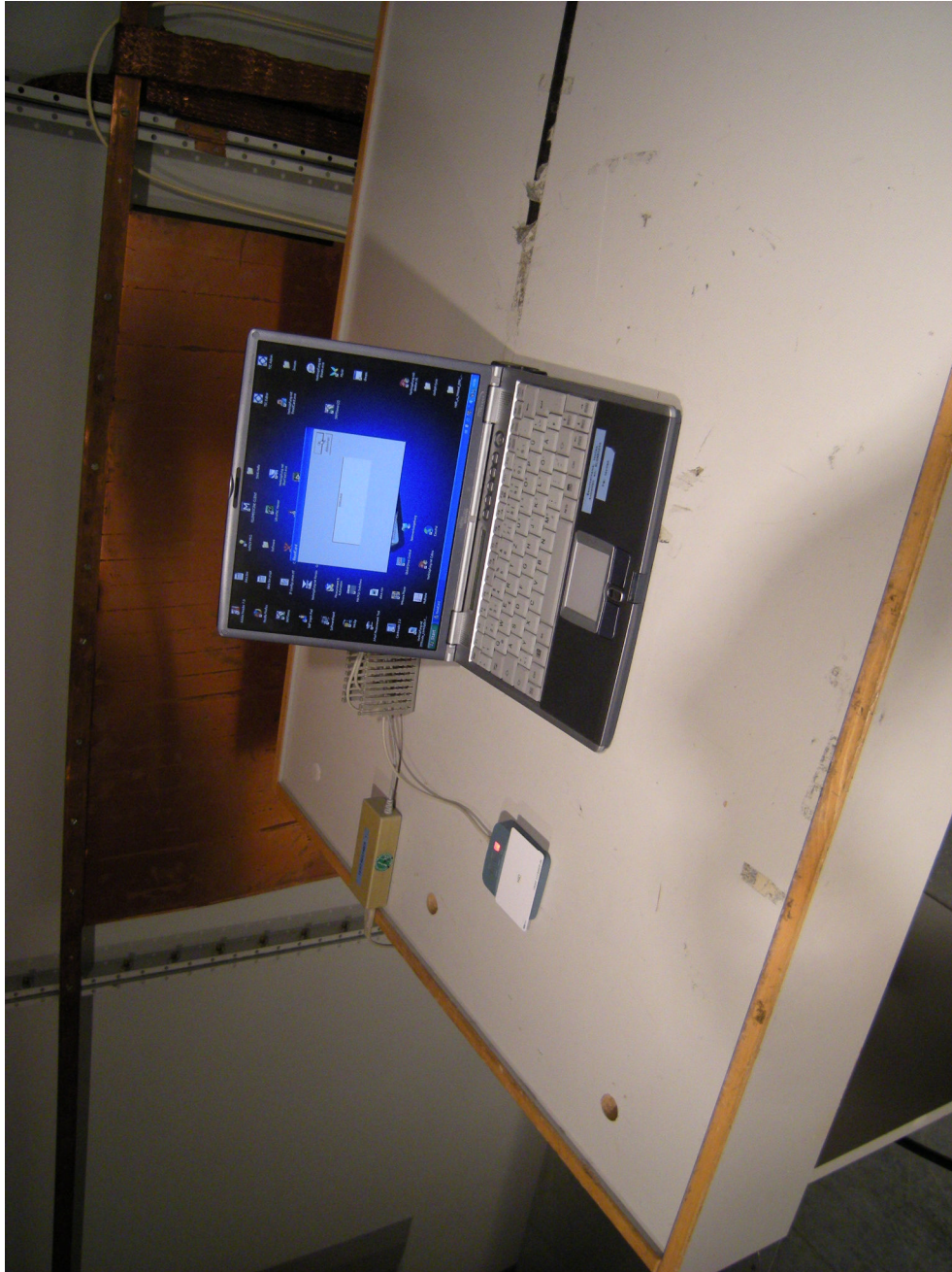
91053emi_c1.jpg: Test set-up conducted emissions
