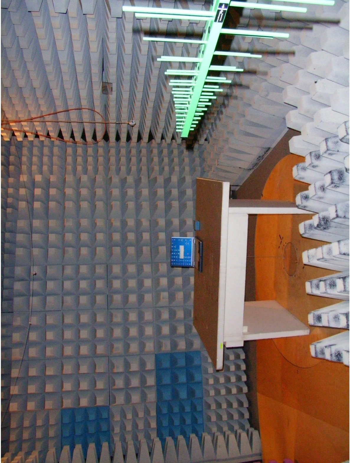
82825emi2.jpg Test set-up fully anechoic chamber (E-Field)
