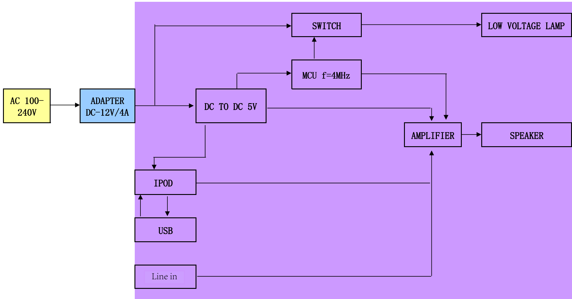
Block Diagram
