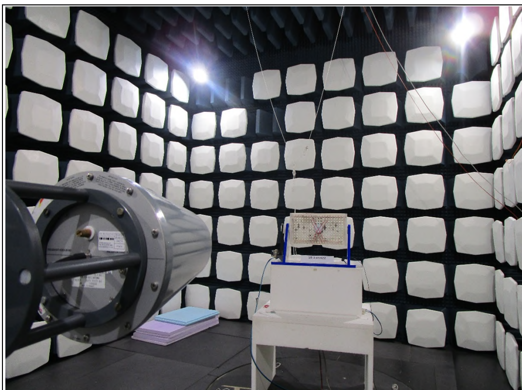
Photograph 4: Radiated measurements test set-up, 1 GHz – 26 GHz
