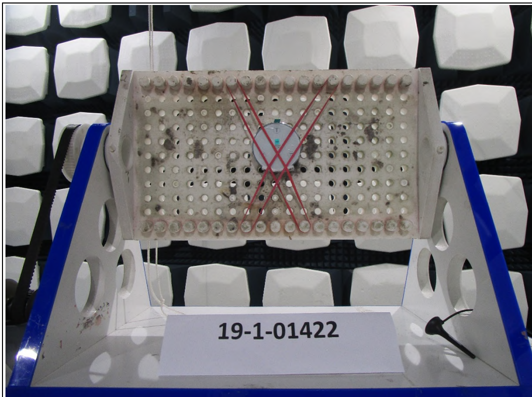
Photograph 3: Radiated measurements test set-up, 1 GHz – 26 GHz
