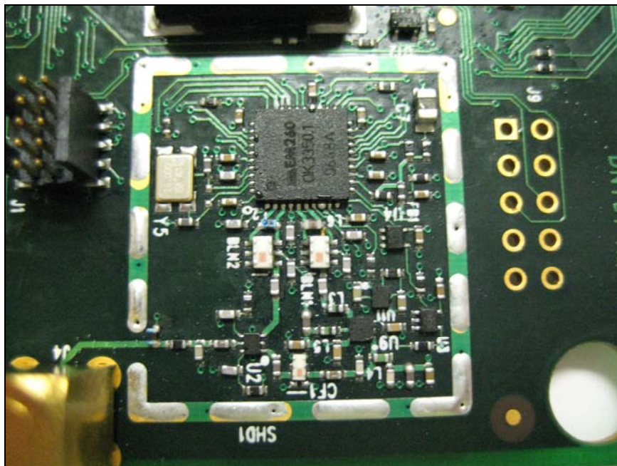
Close up of RF Section – Shield Removed - View #2
