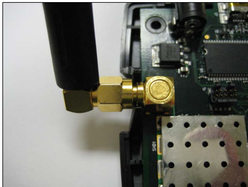
Close Up of Antenna Connection
