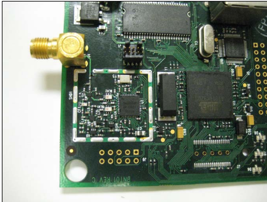
RF Section – Shield Removed - View #1
