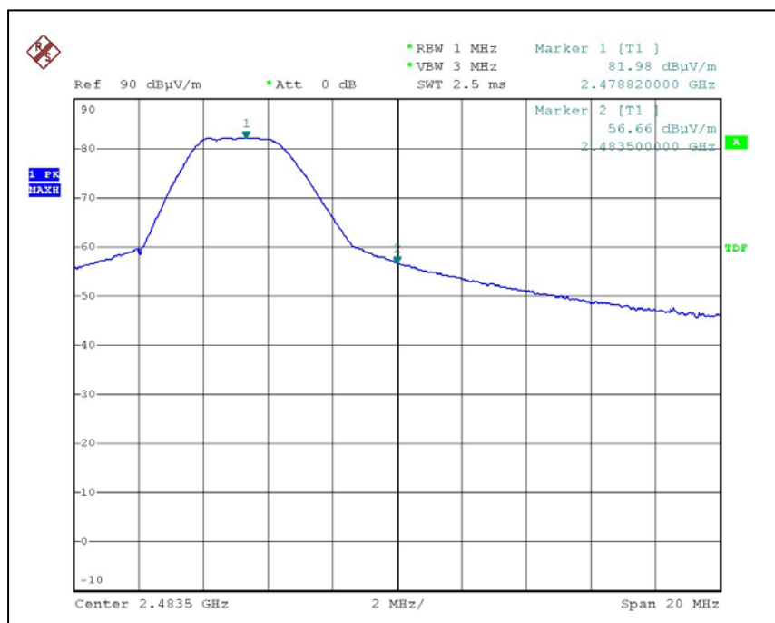
Bandwidth 3 (2.4835GHz Edge with Peak Detector)
