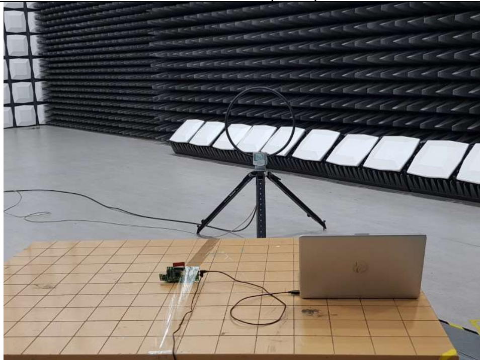
9 kHz – 30 MHz (BT)
