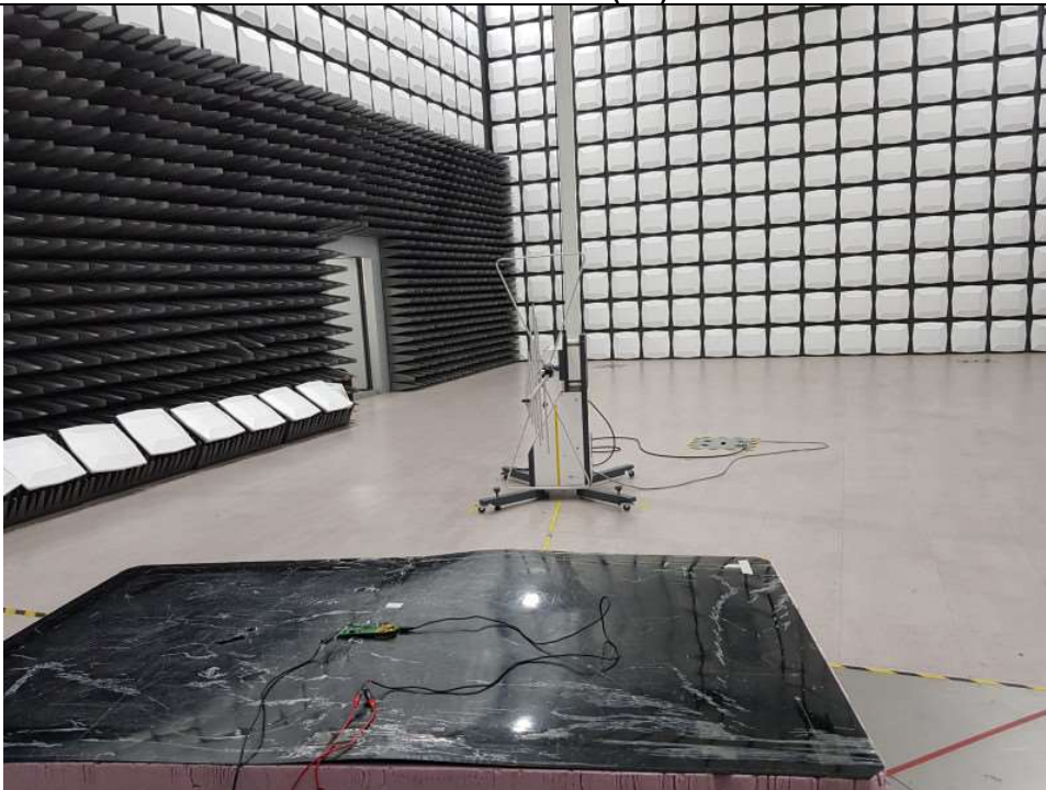
30 MHz – 1 GHz (BT)
