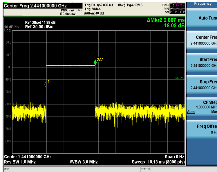
2DH5-Ant1-Hop-PASS
