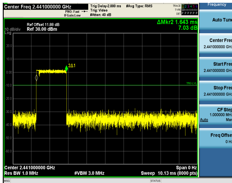
3DH3-Ant1-Hop-PASS
