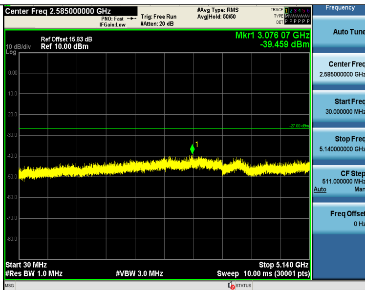
11AC40SISO-Ant1-5190-30~5140-PASS
