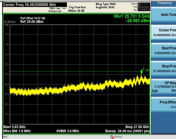
11N20SISO-Ant1-5785-5925~27000-PASS
