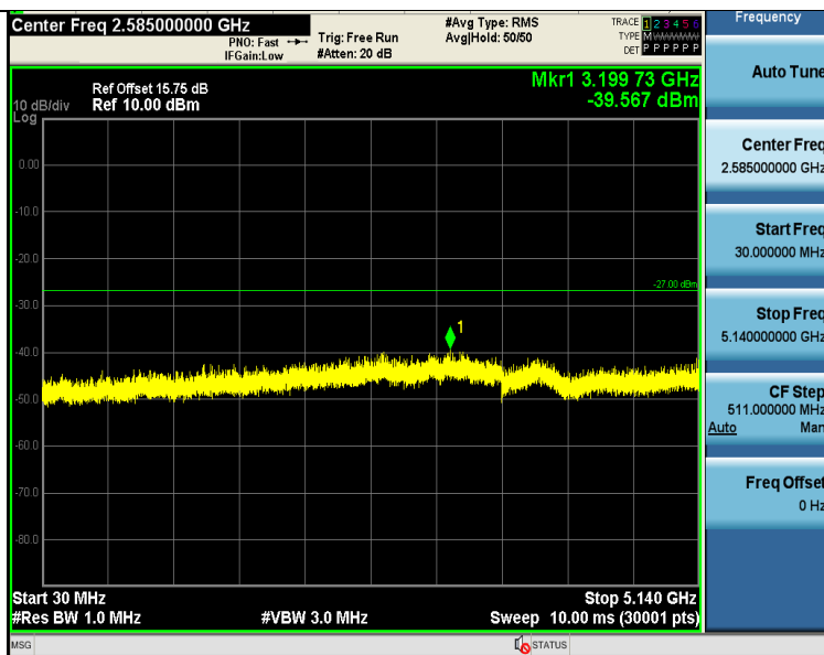
11AC20SISO-Ant1-5180-30~5140-PASS
