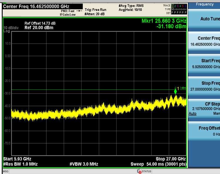
11N40SISO-Ant1-5755-5925~27000-PASS
