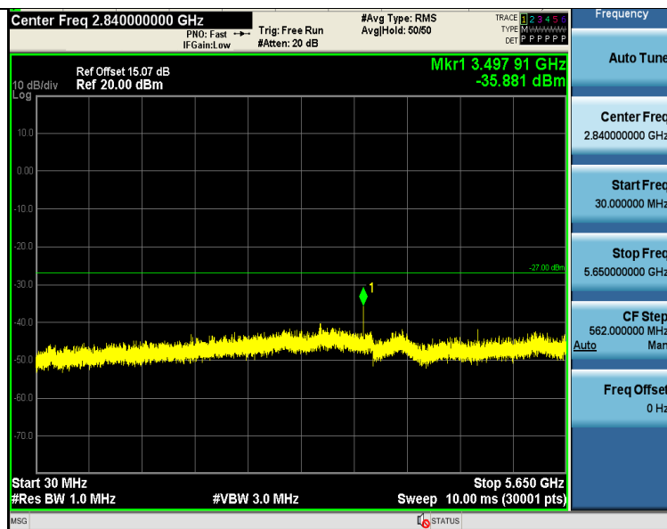
11A-Ant1-5785-30~5650-PASS
