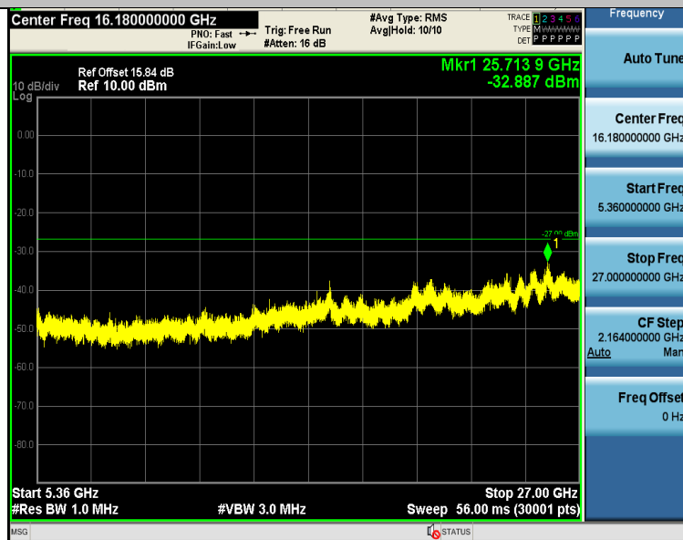
11N20SISO-Ant1-5200-5360~27000-PASS
