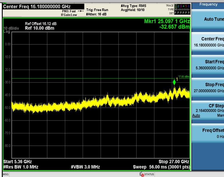
11AC40SISO-Ant1-5230-5360~27000-PASS
