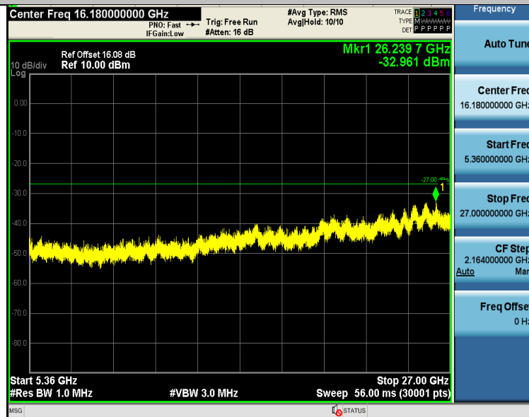
11AC20SISO-Ant1-5240-5360~27000-PASS
