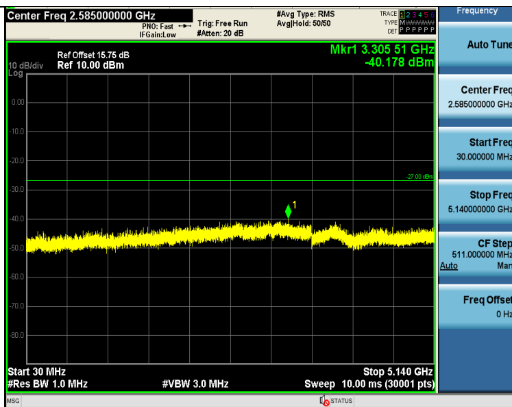
11N20SISO-Ant1-5180-30~5140-PASS
