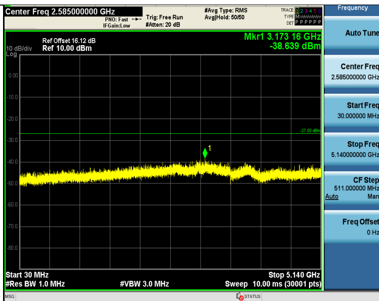
11AC40SISO-Ant1-5230-30~5140-PASS
