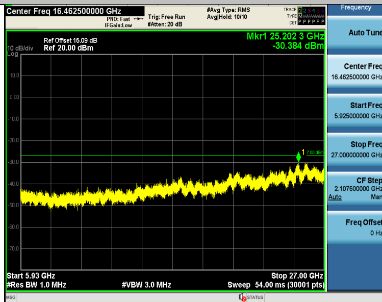
11AC20SISO-Ant1-5825-5925~27000-PASS
