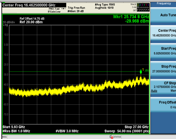
11A-Ant1-5745-5925~27000-PASS
