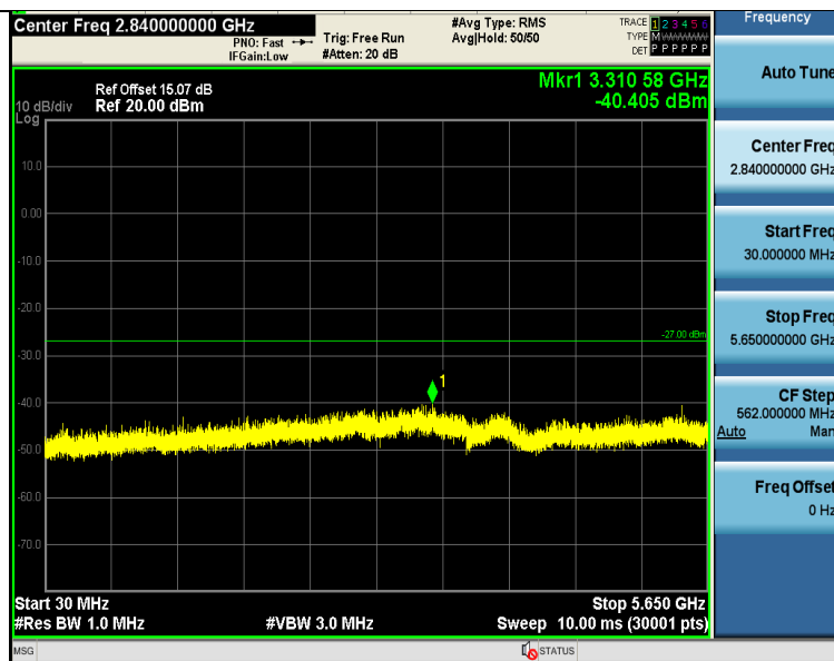
11AC20SISO-Ant1-5785-30~5650-PASS
