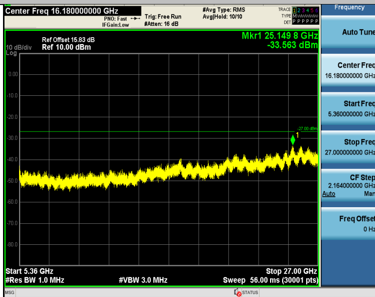
11AC40SISO-Ant1-5190-5360~27000-PASS
