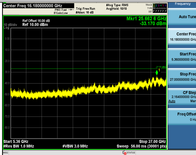
11N20SISO-Ant1-5240-5360~27000-PASS
