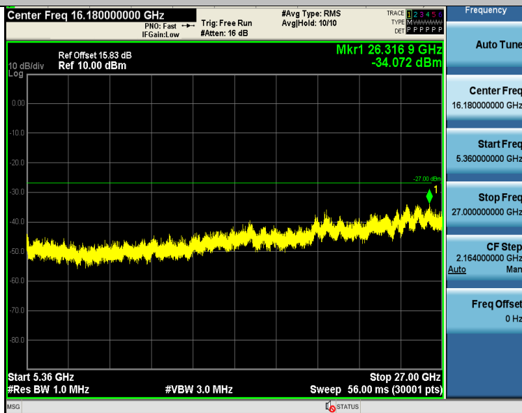
11N40SISO-Ant1-5190-5360~27000-PASS
