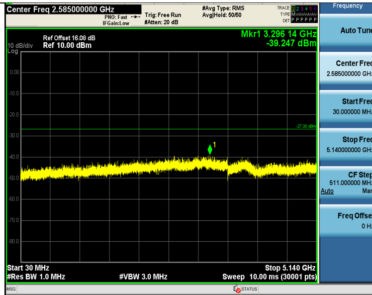
11AC20SISO-Ant1-5240-30~5140-PASS
