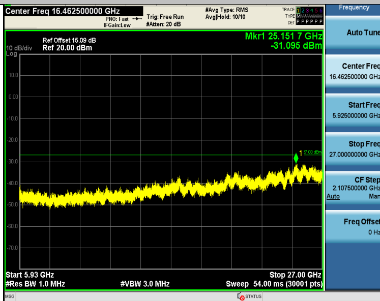
11N20SISO-Ant1-5825-5925~27000-PASS
