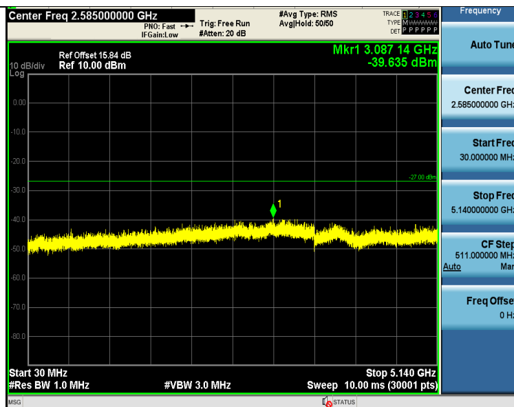
11AC20SISO-Ant1-5200-30~5140-PASS
