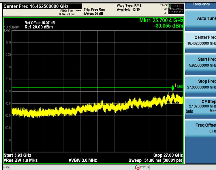
11A-Ant1-5785-5925~27000-PASS
