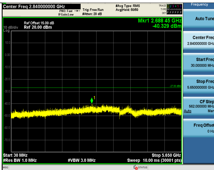
11N20SISO-Ant1-5825-30~5650-PASS
