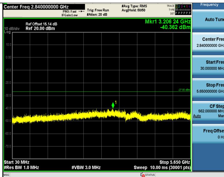
11N40SISO-Ant1-5795-30~5650-PASS
