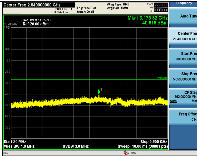
11N20SISO-Ant1-5745-30~5650-PASS
