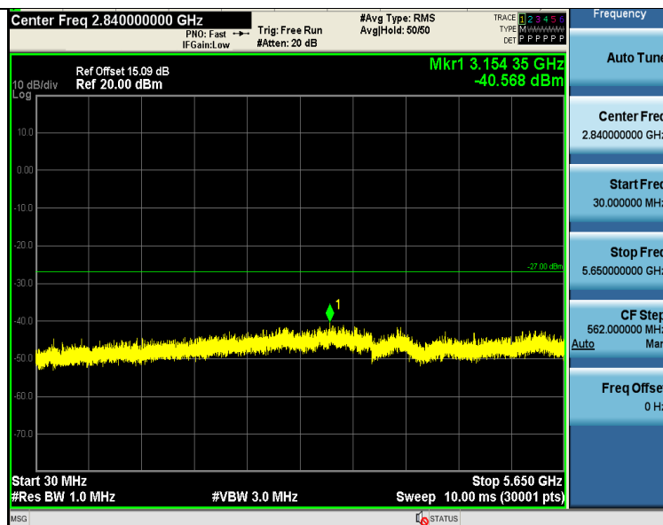
11A-Ant1-5825-30~5650-PASS
