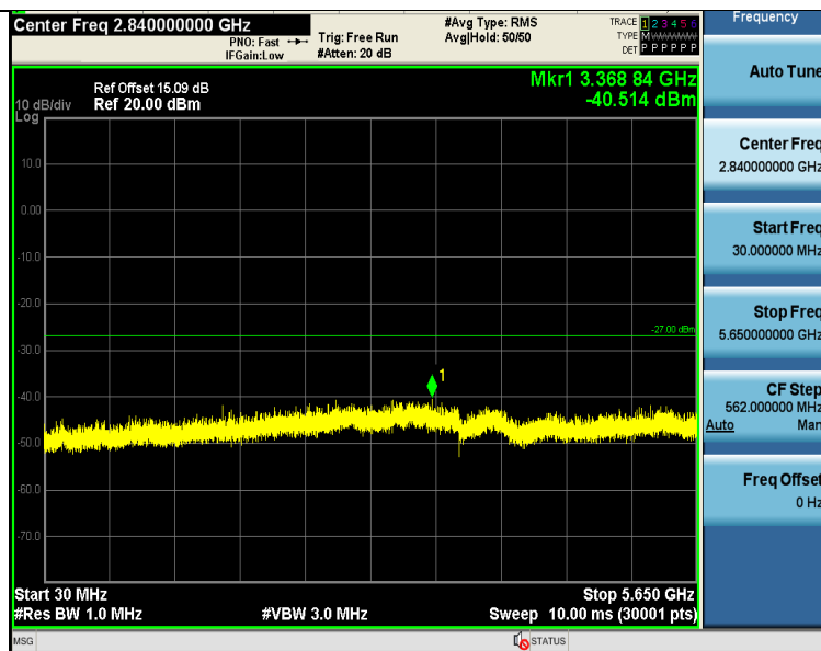
11AC20SISO-Ant1-5825-30~5650-PASS
