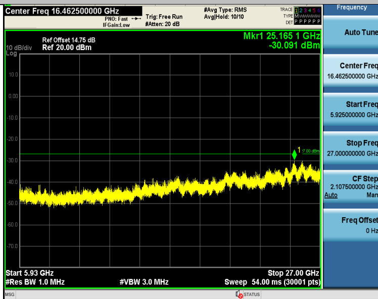
11AC20SISO-Ant1-5745-5925~27000-PASS
