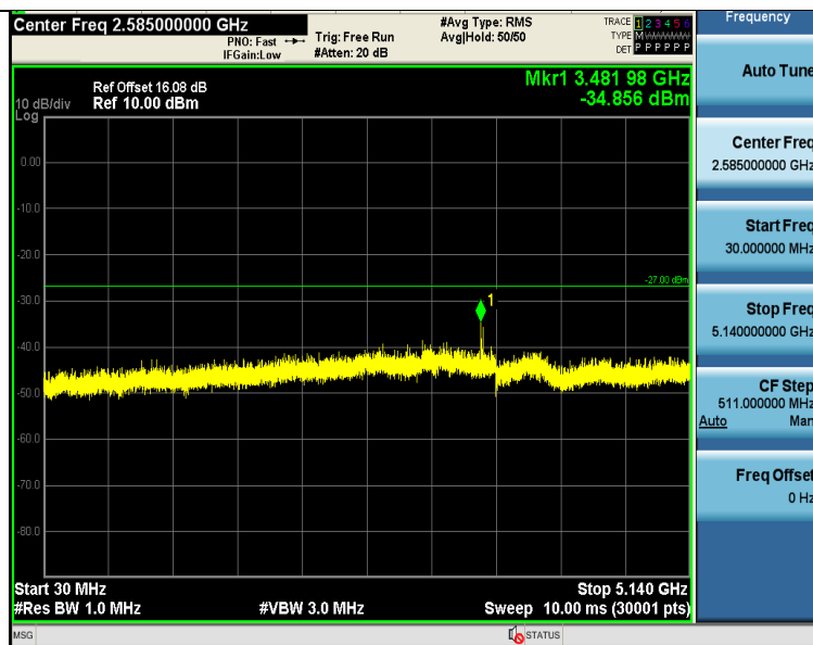
11A-Ant1-5240-30~5140-PASS
