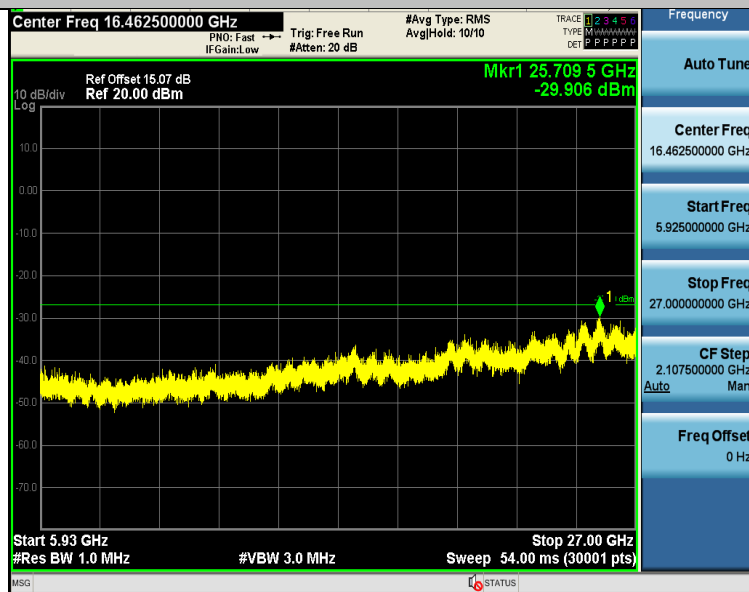
11AC20SISO-Ant1-5785-5925~27000-PASS
