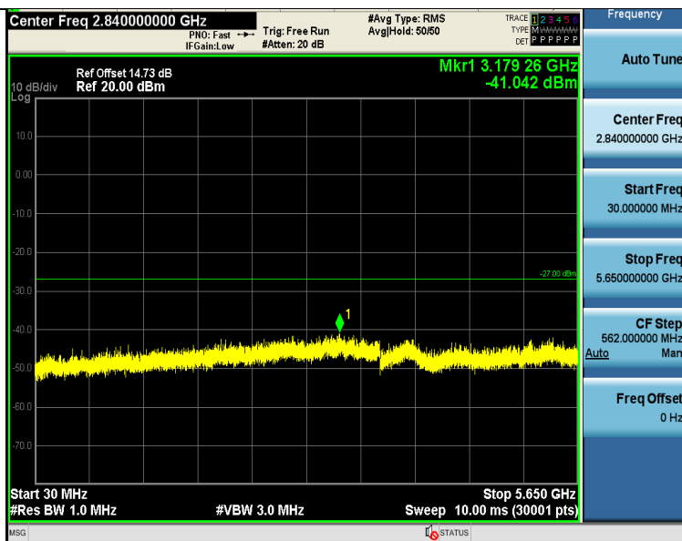
11N40SISO-Ant1-5755-30~5650-PASS
