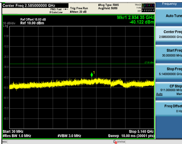
11N40SISO-Ant1-5190-30~5140-PASS
