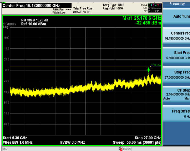
11AC20SISO-Ant1-5180-5360~27000-PASS
