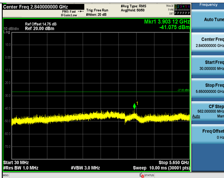
11A-Ant1-5745-30~5650-PASS
