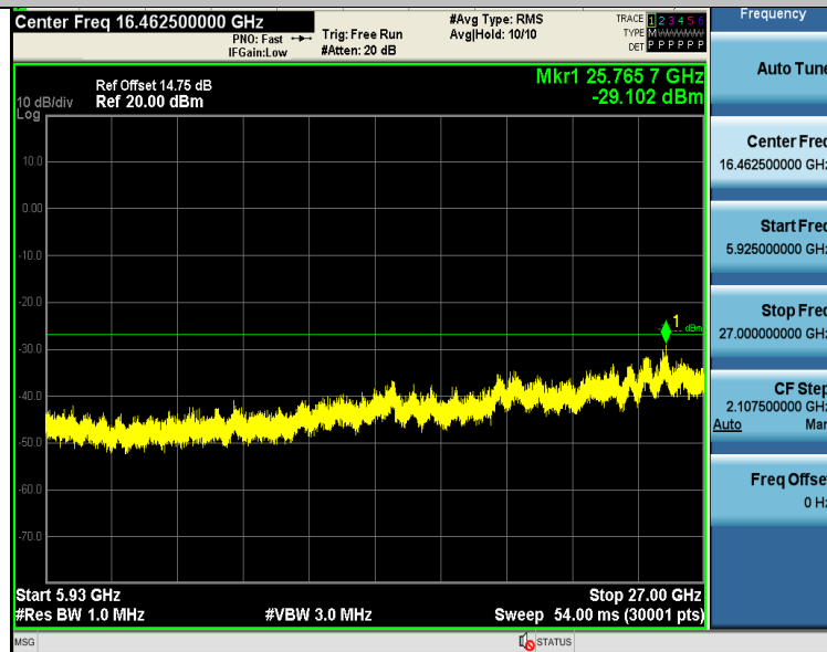
11N20SISO-Ant1-5745-5925~27000-PASS
