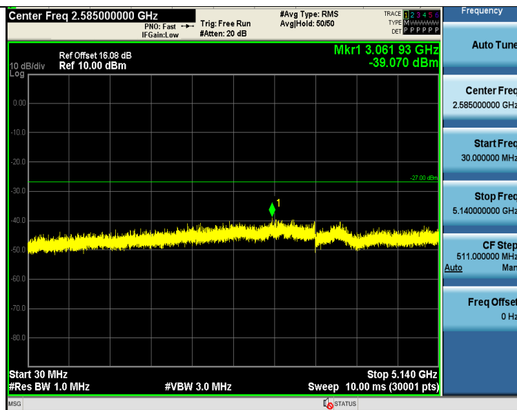
11N20SISO-Ant1-5240-30~5140-PASS
