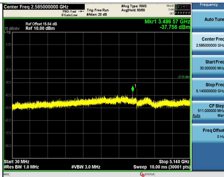
11N20SISO-Ant1-5200-30~5140-PASS
