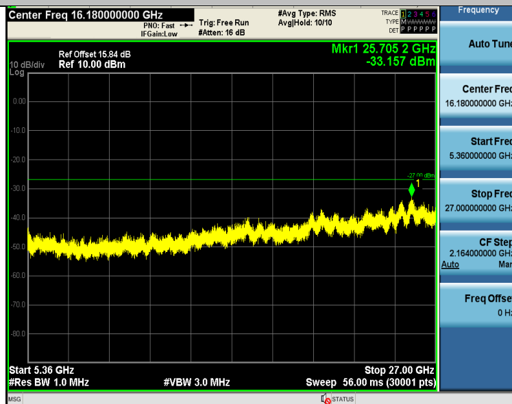
11AC20SISO-Ant1-5200-5360~27000-PASS
