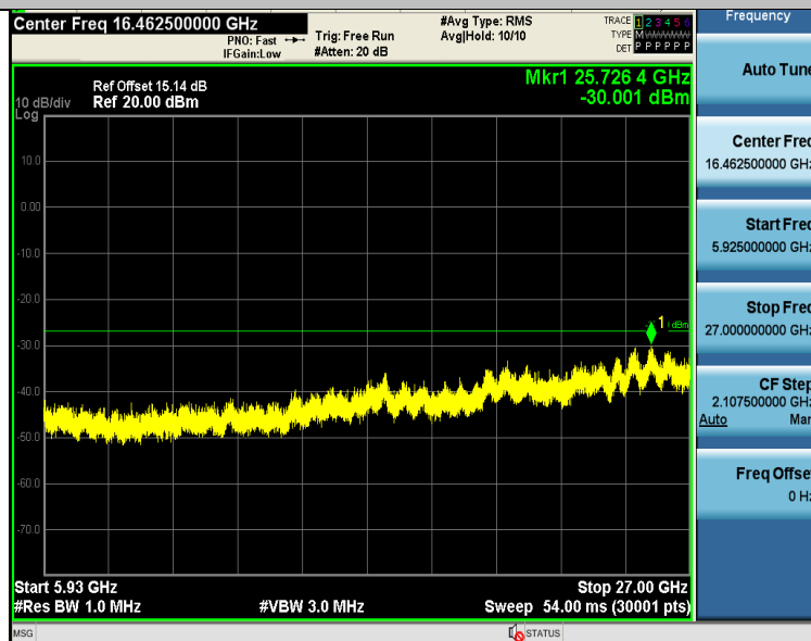
11N40SISO-Ant1-5795-5925~27000-PASS
