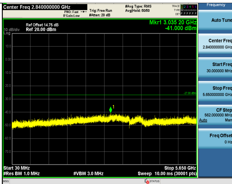
11AC20SISO-Ant1-5745-30~5650-PASS
