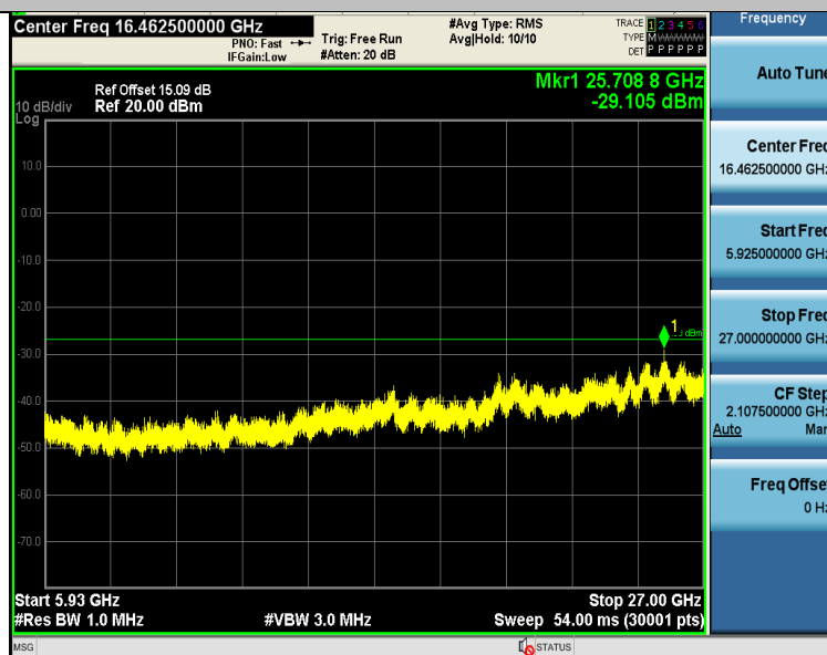
11A-Ant1-5825-5925~27000-PASS
