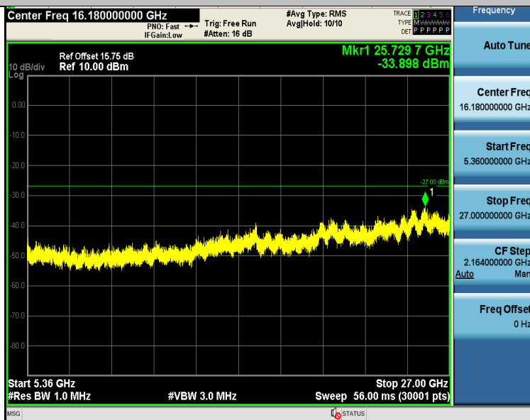
11N20SISO-Ant1-5180-5360~27000-PASS
