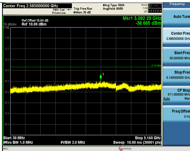
11A-Ant1-5200-30~5140-PASS
