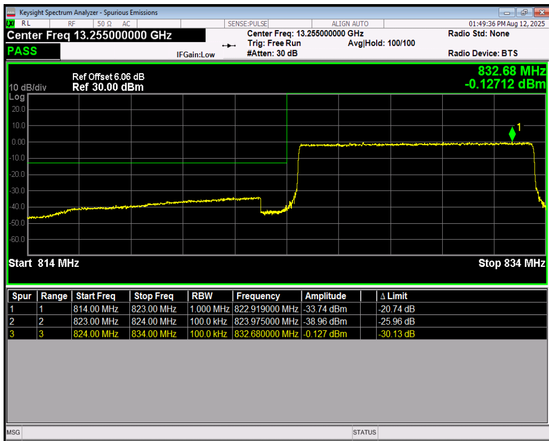
Band5 64QAM BW=10MHz Channel=20450 RB Size=1 Position=#0
