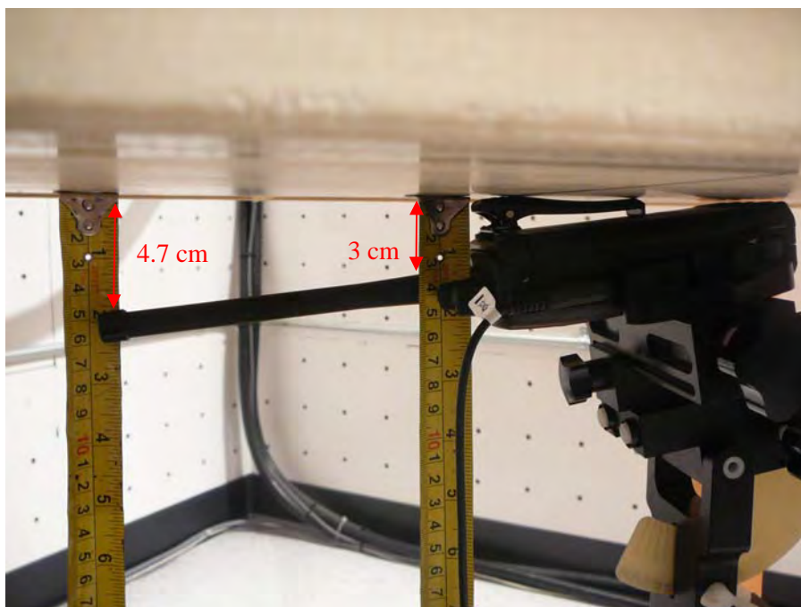
Body Worn - Back Touch to Flat Phantom
