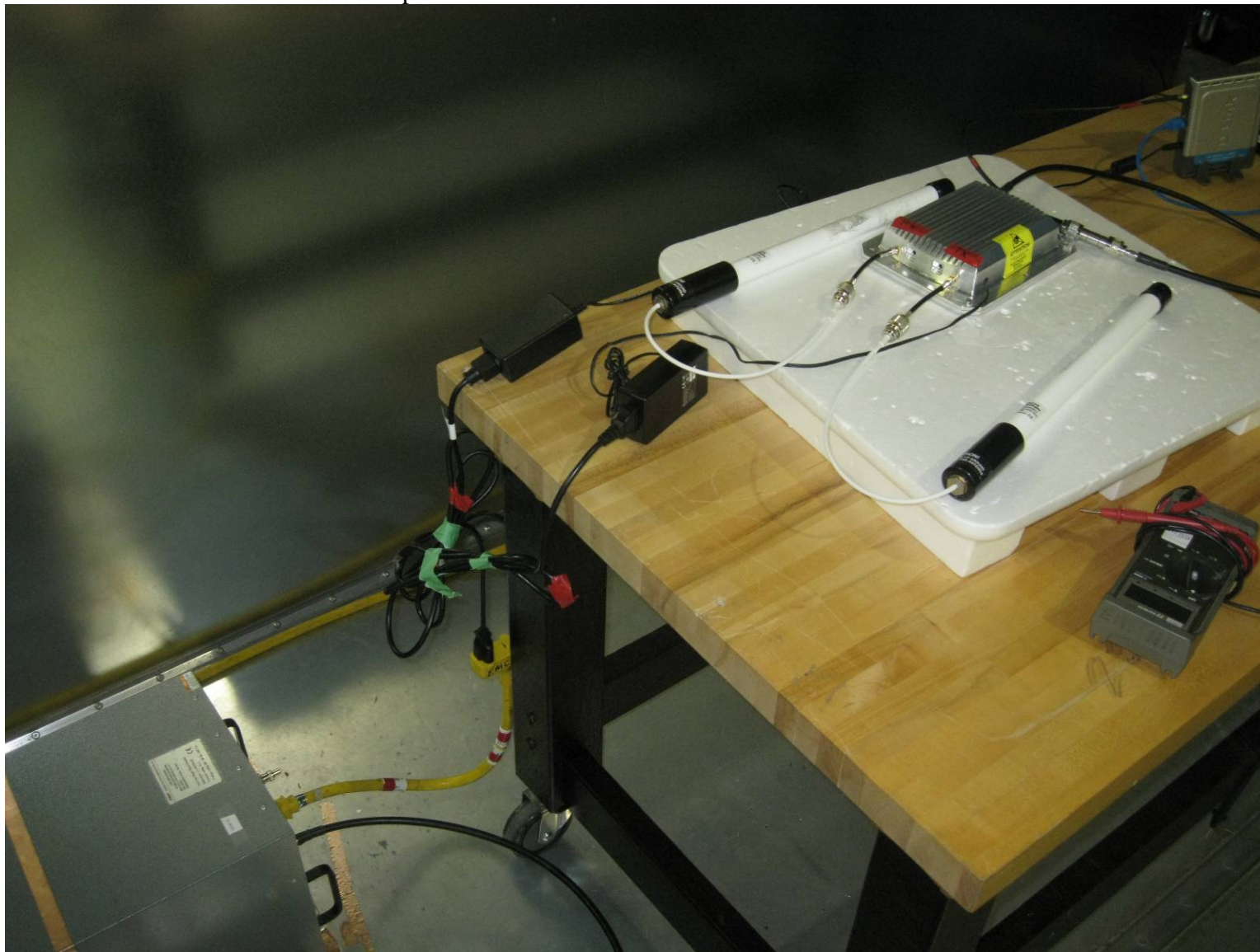
Power line conducted Emissions Setup Photo 2
