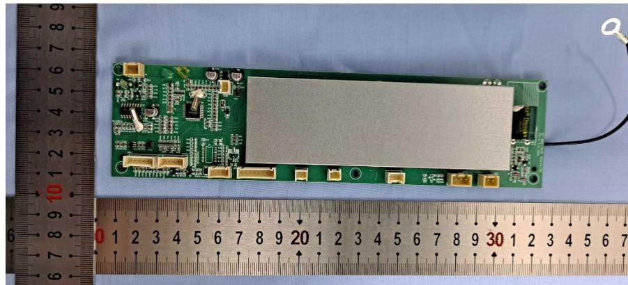
Bild / Picture 10: amplify board
