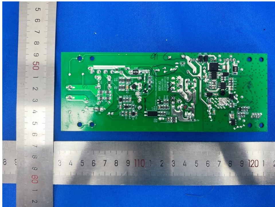
Bild / Picture 13: power board
