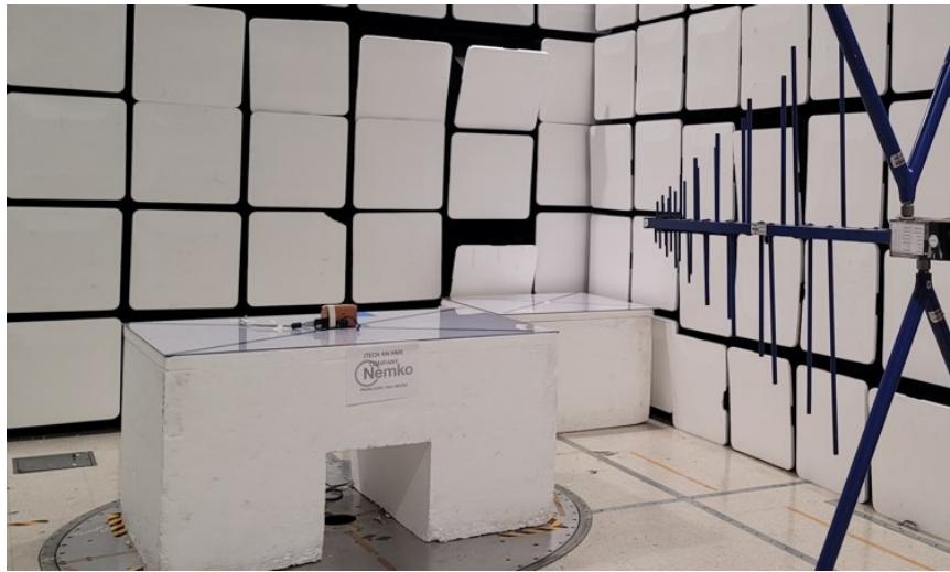
Figure 2 - Radiated emissions below 1 GHz (0.03 – 1 GHz), front view.
