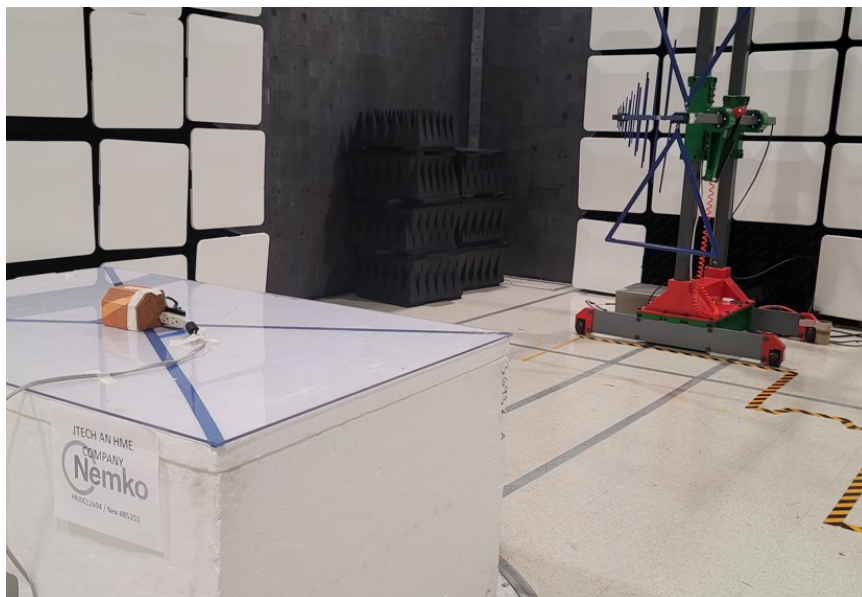
Figure 3 - Radiated emissions below 1 GHz (0.03 – 1 GHz), rear view.
