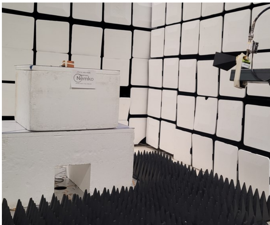
Figure 6 - Radiated emissions above 1 GHz (18 – 26 GHz), front view.
