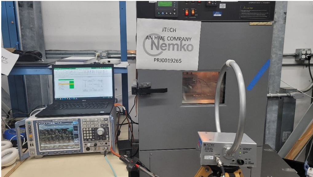
Figure 10 – Test setup, frequency stability.
