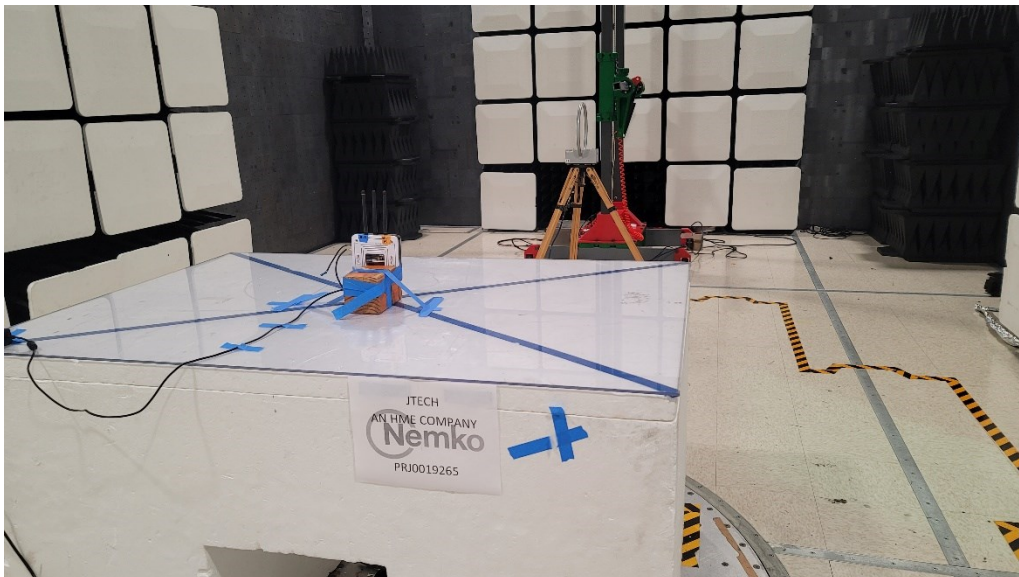
Figure 5 - Radiated emissions below 30 MHz (9 kHz – 30 MHz), 90 Degrees, rear view
