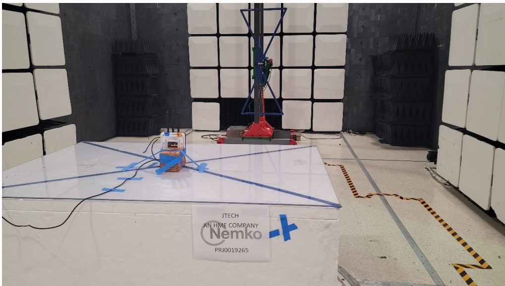
Figure 7 - Radiated emissions below 1 GHz (30 – 150 MHz), rear view.
