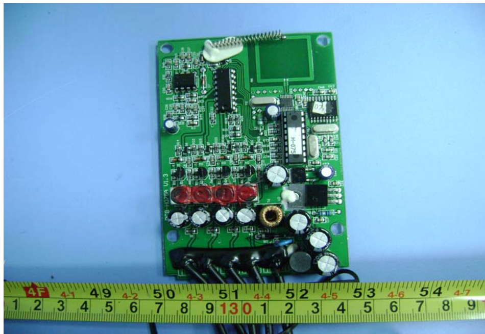
PCB-Front View
