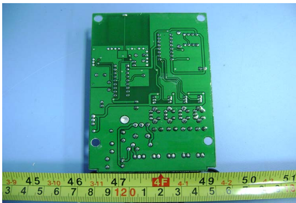
PCB-Back View
