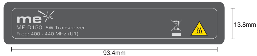
ME-D150 (U1) Top aperture (Produced in factory)
