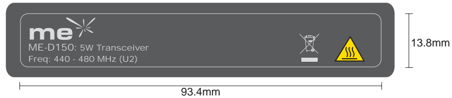
ME-D150 (U2) Top aperture (Produced in factory)
