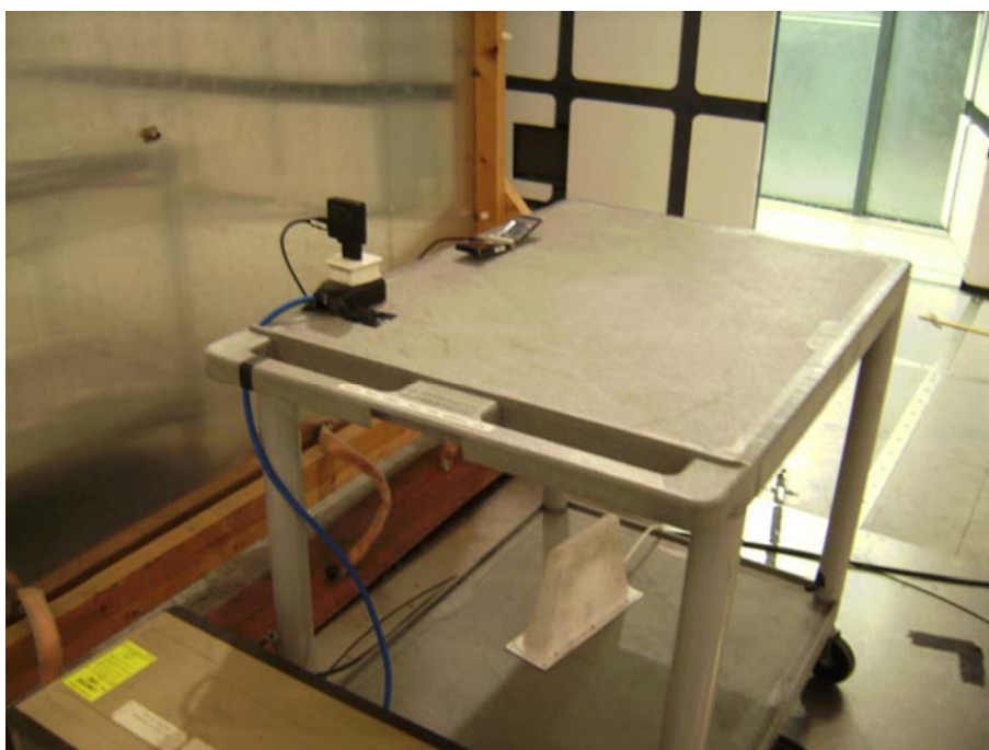
Conducted Emissions (AC Power Port) Test Setup
