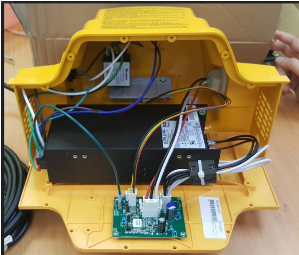
Photograph No.1 WAVE140 POWER SUPPLY Internal view
