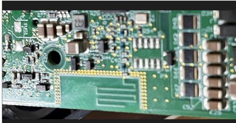
Photograph No.3 Wireless Robotic Pool Cleaner with Inductive Charger Antenna assembly
