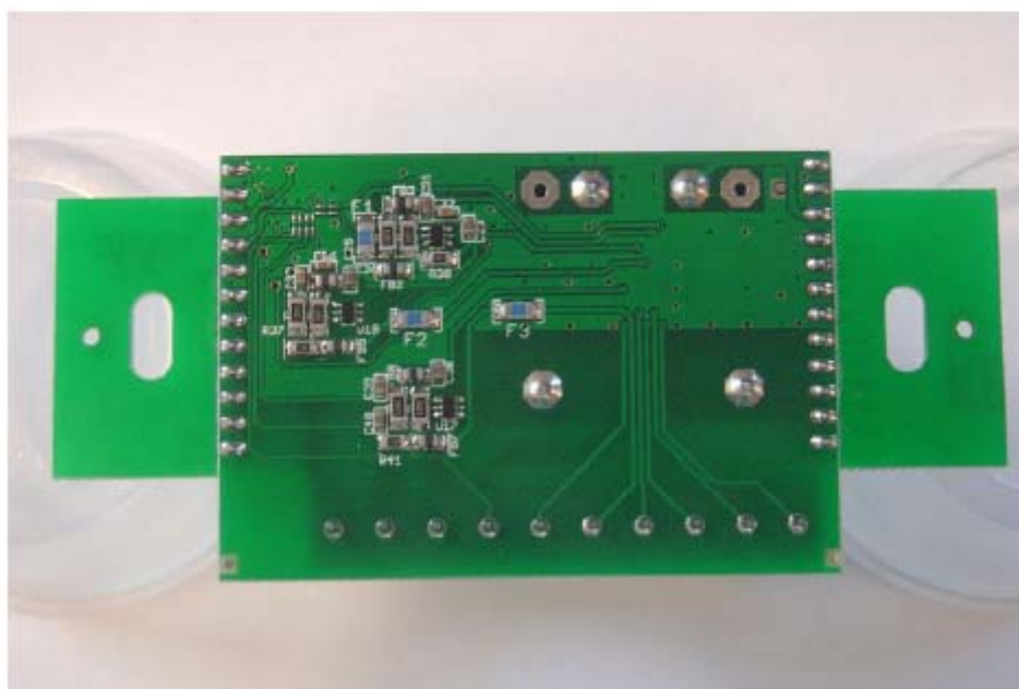
Figure 4. bottom view, PCB - enclosure removed.
