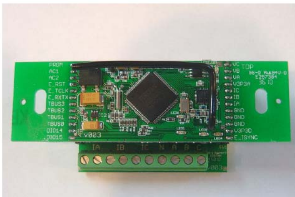
Figure 3. Top view, PCB - enclosure removed.
