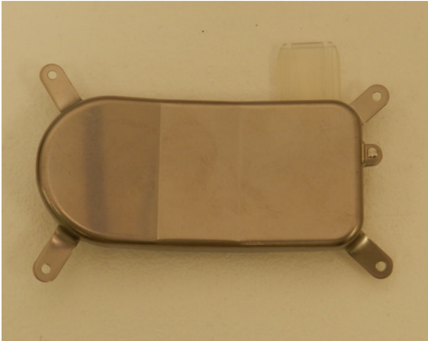
Neurostimulator in a Ferrule with Connector Cover and Lead Strain Relief - Bottom View
