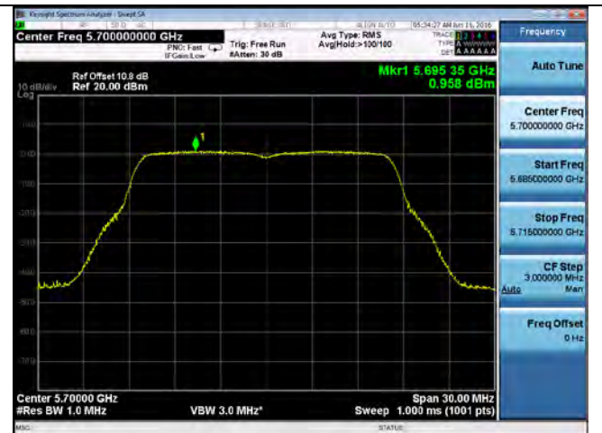
PSD-802.11a-5700M-chain1
