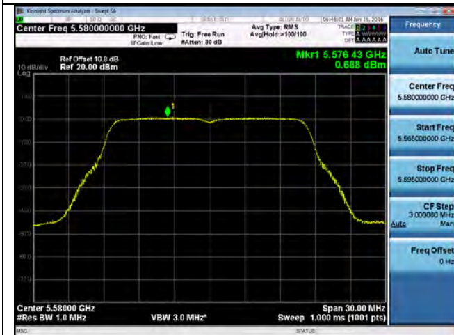
PSD-802.11a-5580M-chain3
