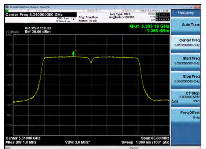
PSD-802.11n-40M-5310M-chain3
