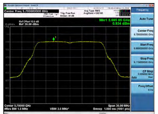
PSD-802.11a-5700M-chain3
