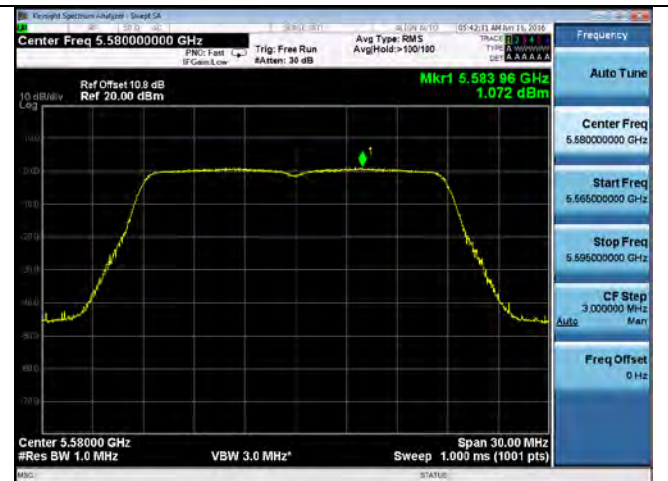
PSD-802.11n-20-5580M-chain1
