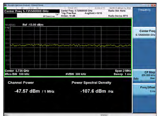
Band Edge -802.11n-20M -5700M-chain3
