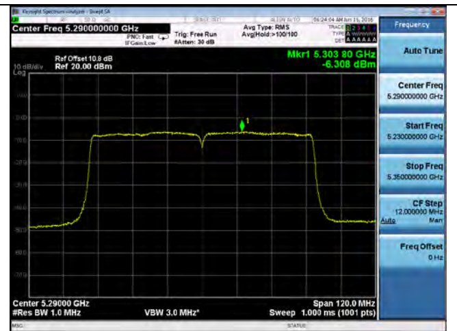
PSD-802.11ac-80M-5290M-chain2
