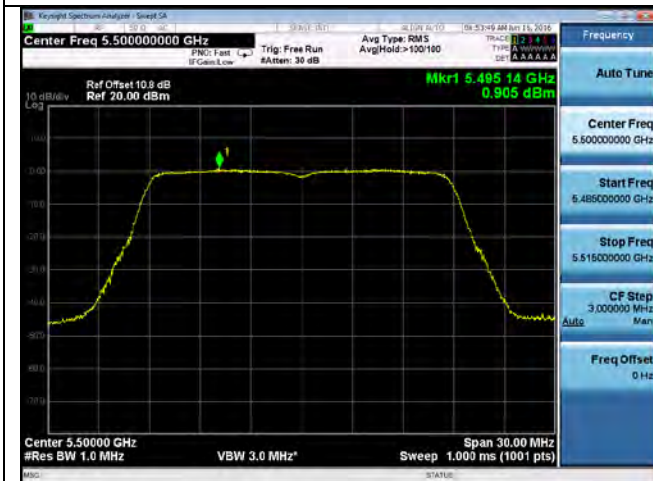
PSD-802.11n-20-5500M-chain3
