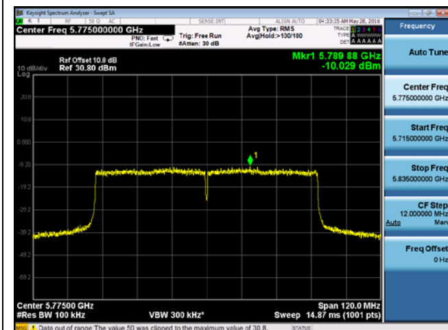
PSD-802.11ac-80-5775M-chain2
