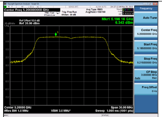
PSD-802.11a-5200M-chain3
