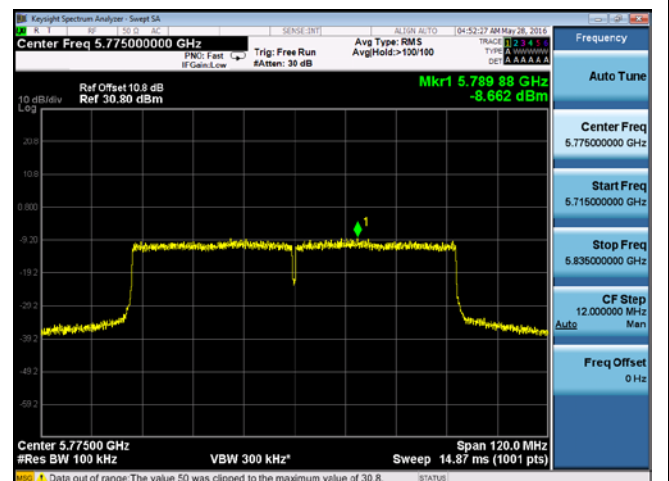
PSD-802.11ac-80-5775M-chain3
