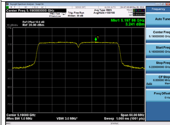
PSD-802.11n-40M-5190M-chain3
