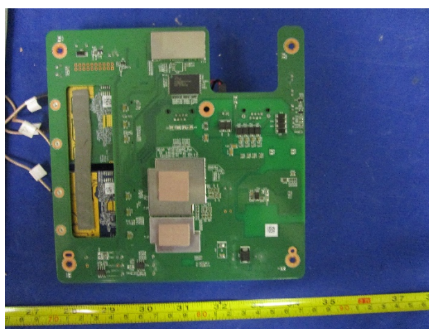
AP PCBA RearView
