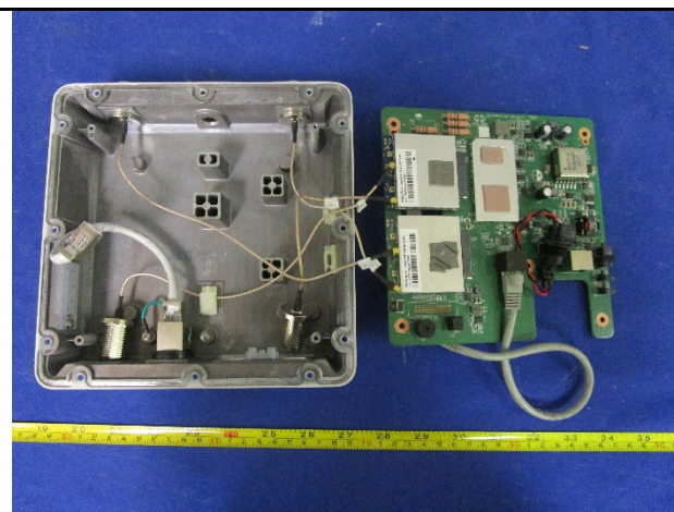
AP View 2
