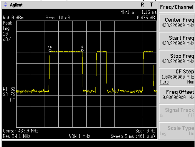
(1.15ms burst: 9pcs)
