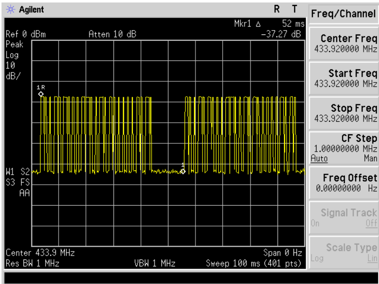
(Transmit cycle 52ms)
