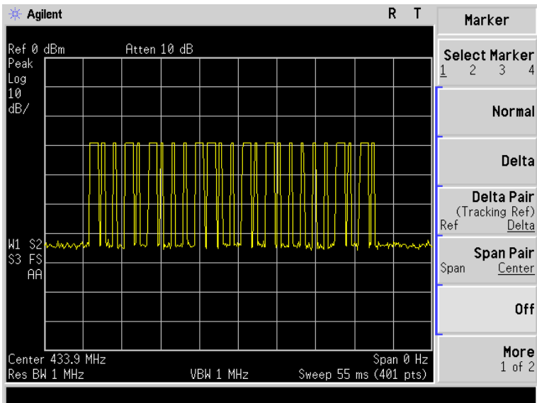
(Total 25pcs Bursts in a transmit cycle)
