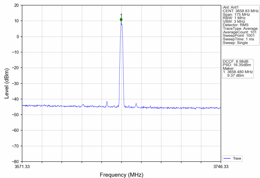
n78d_30kHz_SISO_NTNV_70MHz_CP-OFDM_64_QAM_3624.99MHz_Edge_1RB_Right
