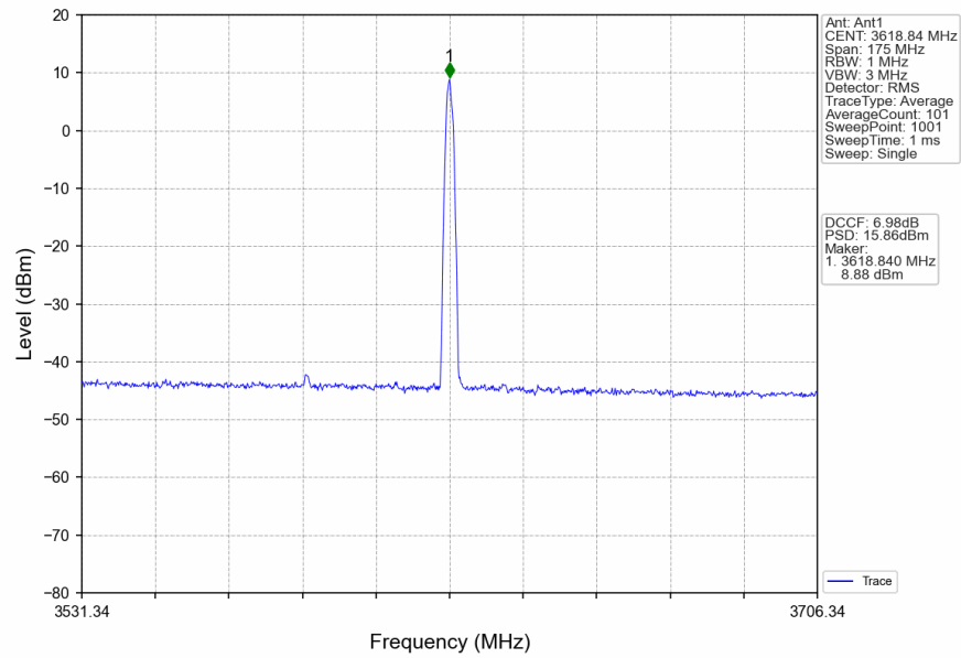
n78d_30kHz_SISO_NTNV_70MHz_CP-OFDM_64_QAM_3585MHz_Edge_1RB_Right
