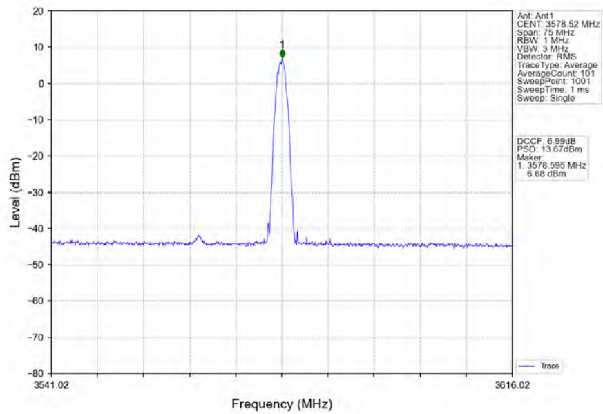
n78d_30kHz_SISO_NTNV_30MHz_DFT-s-OFDM_16_QAM_3565.02MHz_Inner_1RB_Right
