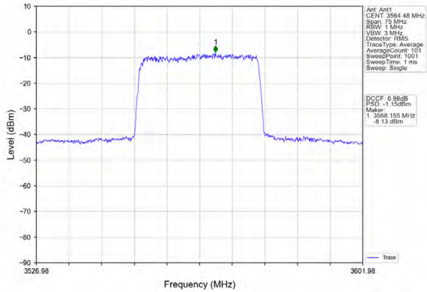
n78d_30kHz_SISO_NTNV_30MHz_DFT-s-OFDM_256_QAM_3565.02MHz_Inner_Full
