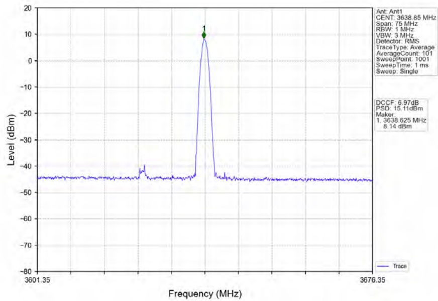
n78d_30kHz_SISO_NTNV_30MHz_DFT-s-OFDM_16_QAM_3624.99MHz_Edge_1RB_Right
