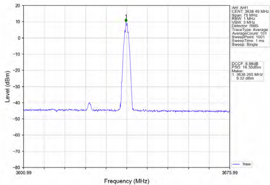
n78d_30kHz_SISO_NTNV_30MHz_CP-OFDM_256_QAM_3624.99MHz_Inner_1RB_Right
