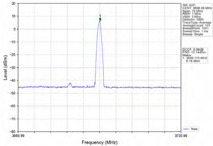
n78d_30kHz_SISO_NTNV_30MHz_CP-OFDM_QPSK_3684.99MHz_Inner_1RB_Right
