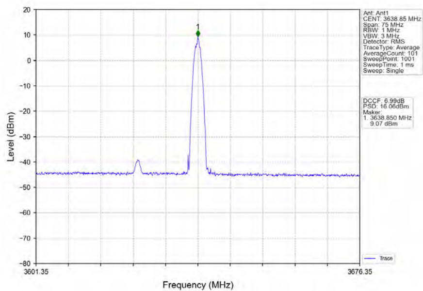
n78d_30kHz_SISO_NTNV_30MHz_CP-OFDM_256_QAM_3624.99MHz_Edge_1RB_Right
