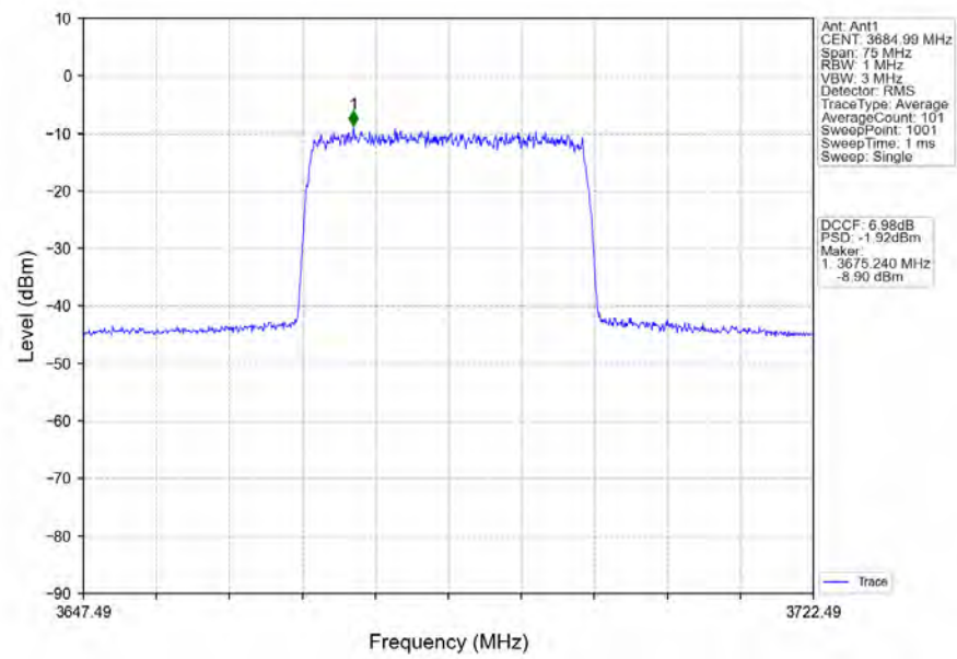
n78d_30kHz_SISO_NTNV_30MHz_CP-OFDM_16_QAM_3684.99MHz_Inner_Full
