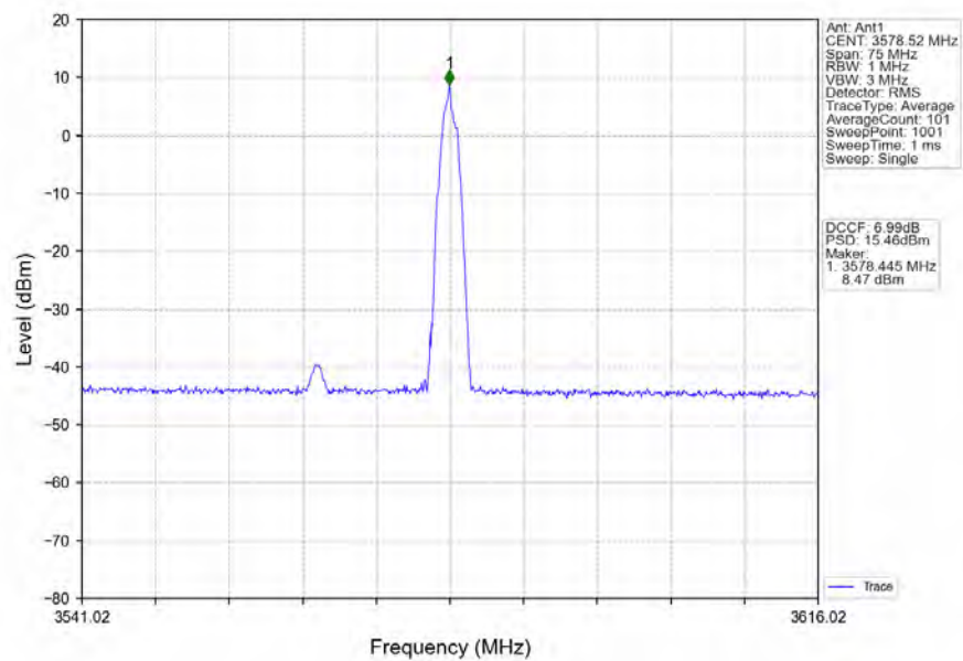
n78d_30kHz_SISO_NTNV_30MHz_CP-OFDM_16_QAM_3565.02MHz_Inner_1RB_Right
