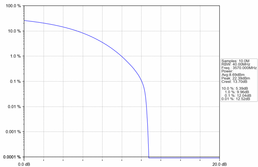
n78d_30kHz_SISO_NTNV_40MHz_CP-OFDM_QPSK_3570MHz_Outer_Full
