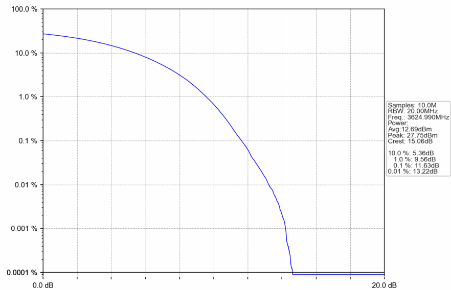
n78d_30kHz_SISO_NTNV_20MHz_CP-OFDM_256_QAM_3624.99MHz_Outer_Full
