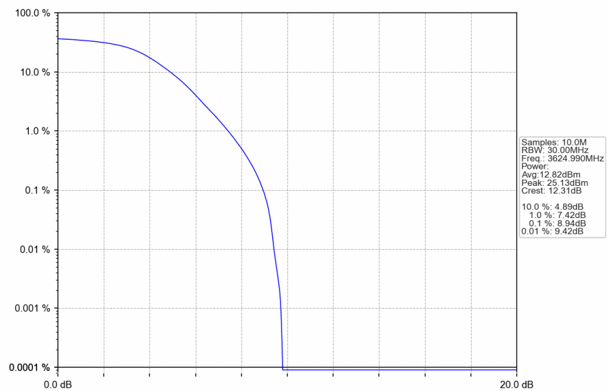
n78d_30kHz_SISO_NTNV_30MHz_DFT-s-OFDM_QPSK_3624.99MHz_Outer_Full
