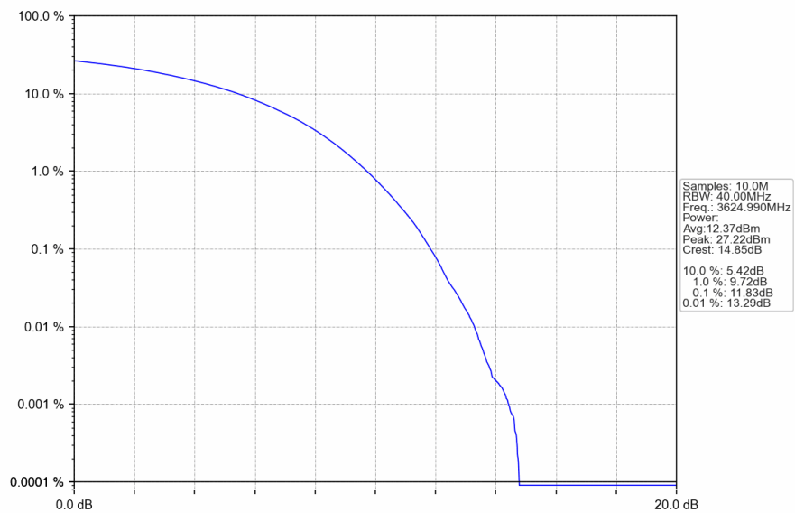
n78d_30kHz_SISO_NTNV_40MHz_CP-OFDM_256_QAM_3624.99MHz_Outer_Full
