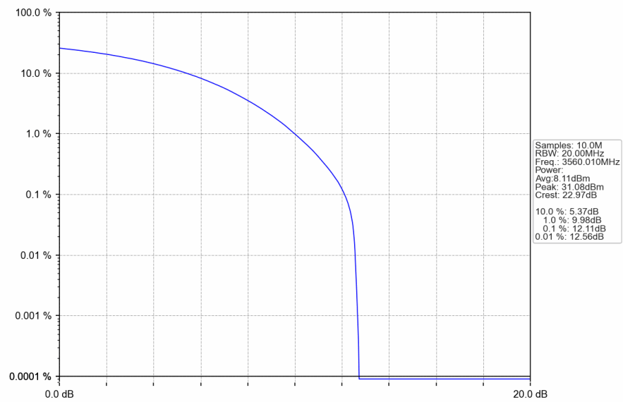
n78d_30kHz_SISO_NTNV_20MHz_CP-OFDM 64 QAM_3560.01MHz_Outer_Full
