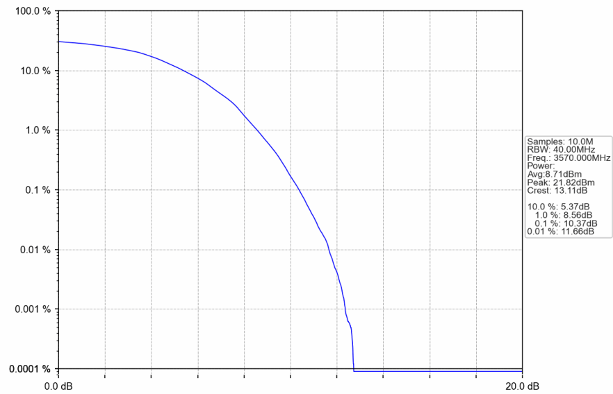
n78d_30kHz_SISO_NTNV_40MHz_DFT-s-OFDM_64_QAM_3570MHz_Outer_Full
