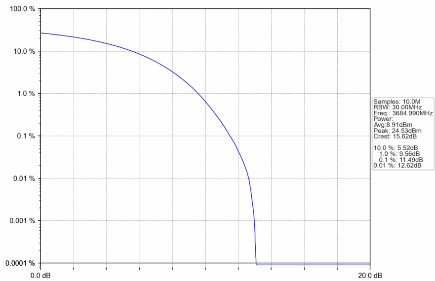
n78d_30kHz_SISO_NTNV_30MHz_CP-OFDM_QPSK_3684.99MHz_Outer_Full
