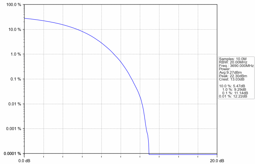
n78d_30kHz_SISO_NTNV_20MHz_CP-OFDM 64 QAM_3690MHz_Outer_Full
