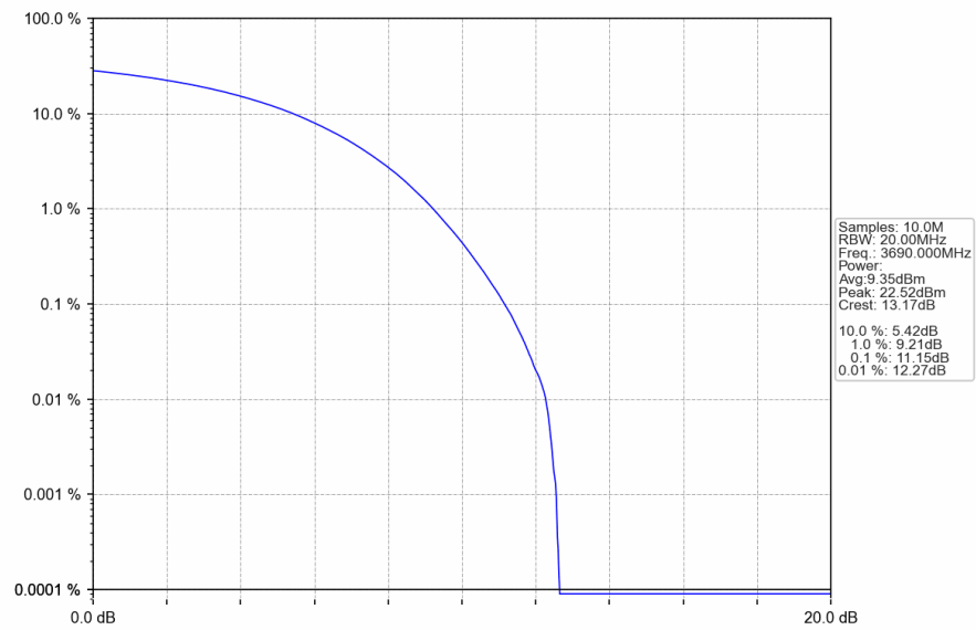
n78d_30kHz_SISO_NTNV_20MHz_CP-OFDM 16 QAM_3690MHz_Outer_Full
