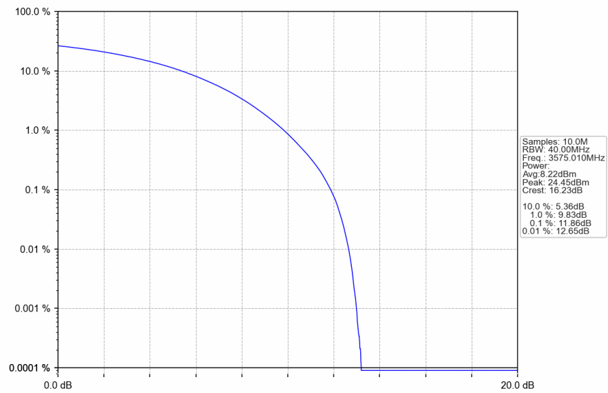
n78d_30kHz_SISO_NTNV_50MHz_CP-OFDM_16_QAM_3575.01MHz_Outer_Full
