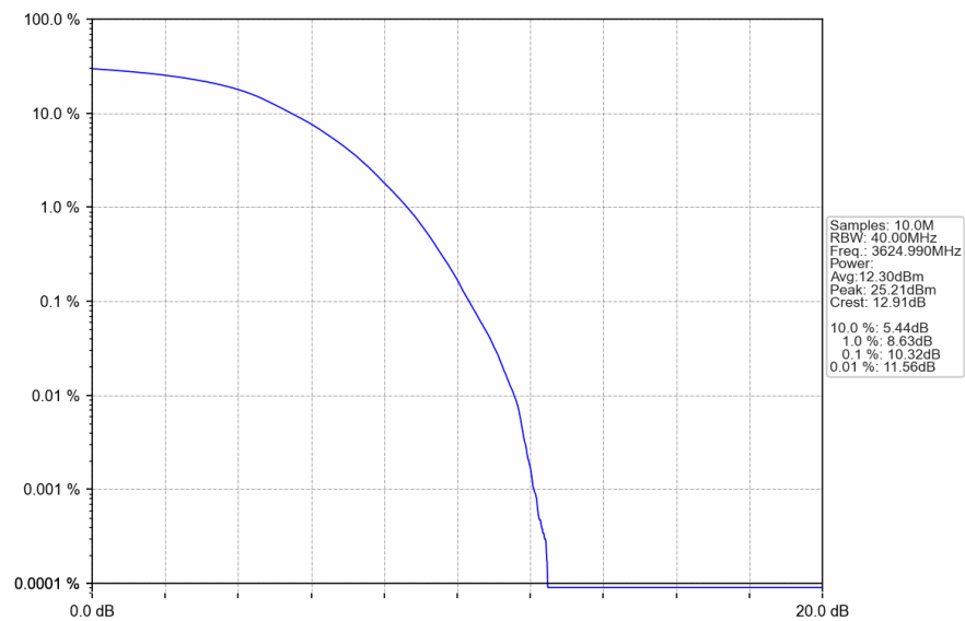
n78d_30kHz_SISO_NTNV_40MHz_DFT-s-OFDM_256_QAM_3624.99MHz_Outer_Full
