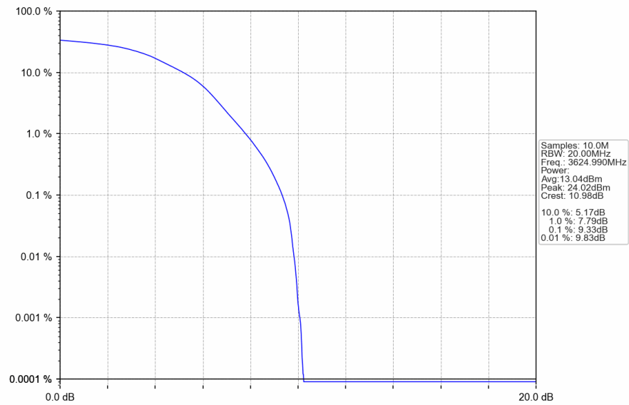
n78d_30kHz_SISO_NTNV_20MHz_DFT-s-OFDM_16_QAM_3624.99MHz_Outer_Full
