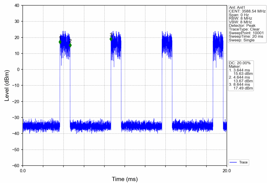
n78d_30kHz_SISO_NTNV_40MHz_CP-OFDM_16 QAM_3570MHz_Inner_1RB_Right
