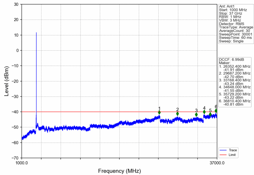
n78d_30kHz_SISO_NTNV_70MHz_DFT-s-OFDM QPSK_3664.98MHz_Edge_1RB_Right
