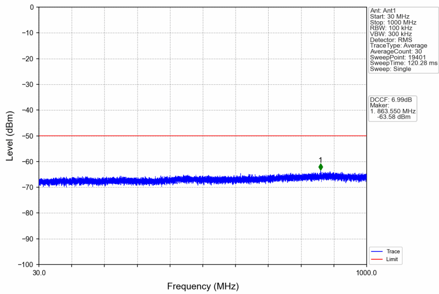
n78d_30kHz_SISO_NTNV_60MHz_DFT-s-OFDM QPSK_3669.99MHz_Edge_1RB_Right
