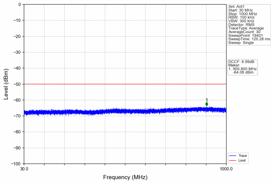
n78d_30kHz_SISO_NTNV_70MHz_DFT-s-OFDM QPSK_3664.98MHz_Edge_1RB_Right
