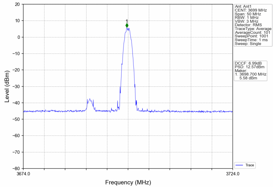
n48_30kHz_SISO_NTNV_20MHz_CP-OFDM_256_QAM_3690MHz_Edge_1RB_Right
