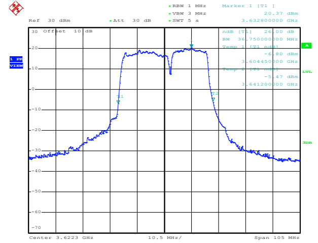
64QAM Low channel
