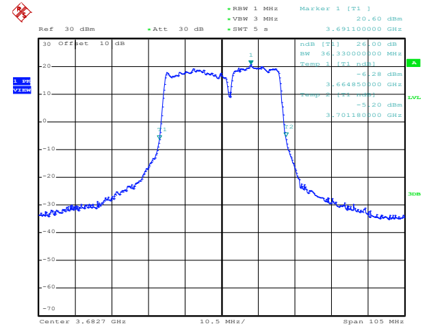
64QAM High channel
