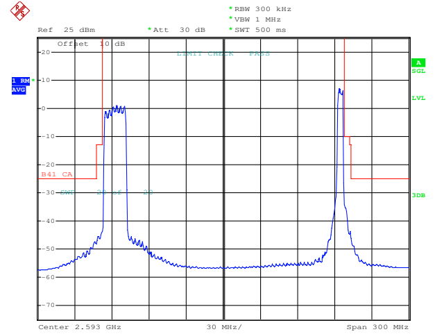
Q64 channel-Full RB offset 0
