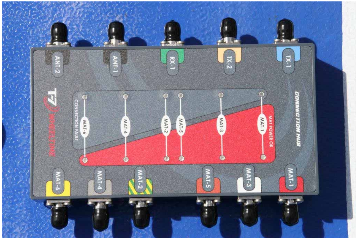
Connection Hub
