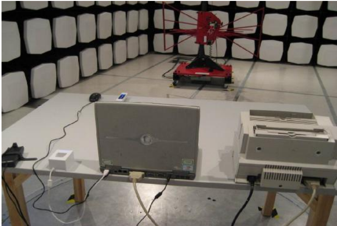
Measurement of Radiated Emission Test Set Up
