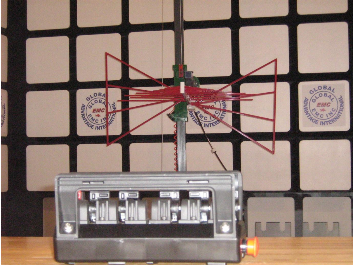
Figure 3 – Radiated emissions
