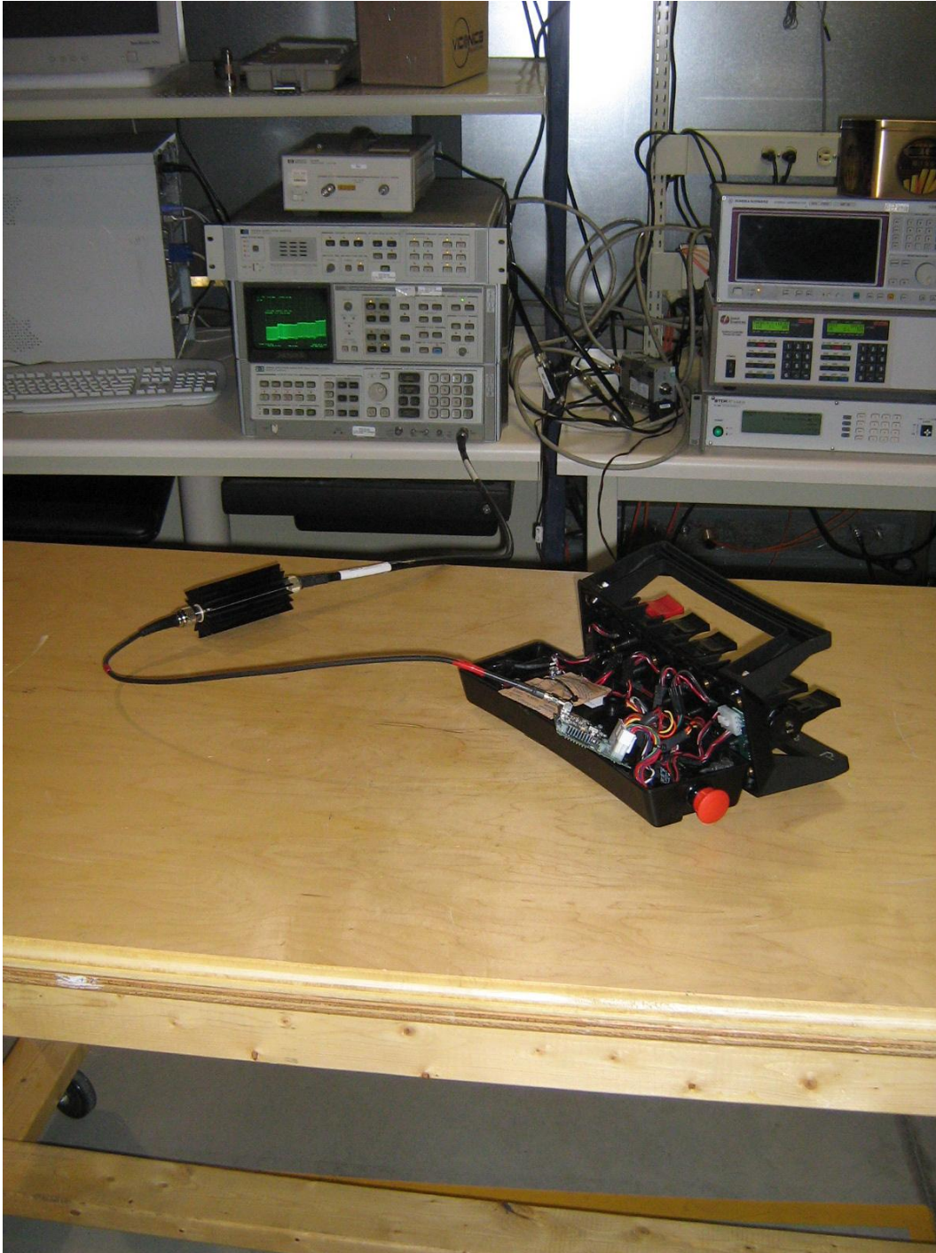
Figure 5 – Antenna port conducted emissions
