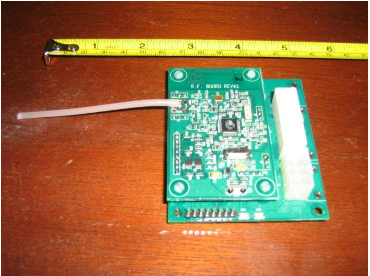
Figure 1 – Transmitter – Front
