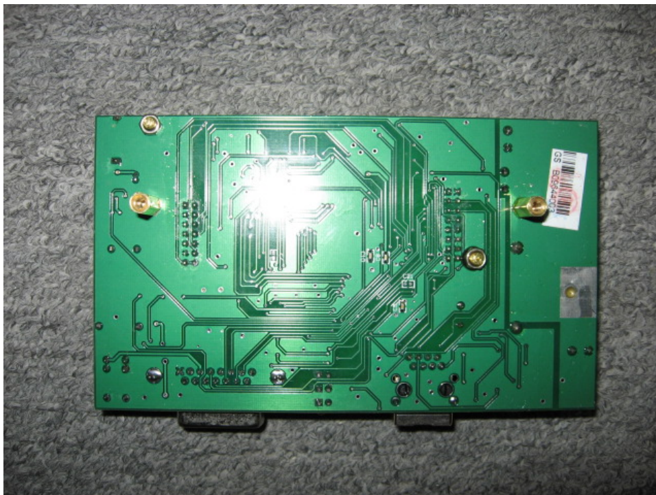
Photo 8 – Back view of Board 2
