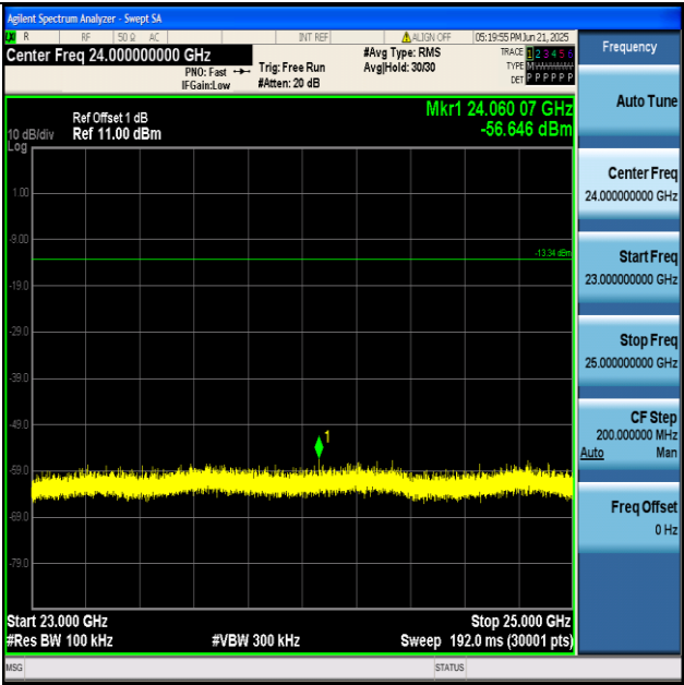
BLE_125K-Ant1-2480-23000~25000-PASS
