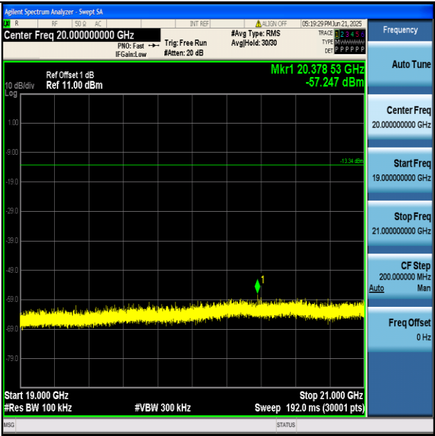
BLE_125K-Ant1-2480-19000~21000-PASS
