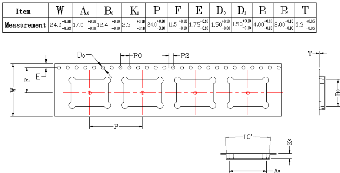
Figure 20. CYBT-2X30XX-02 Tape Dimensions
