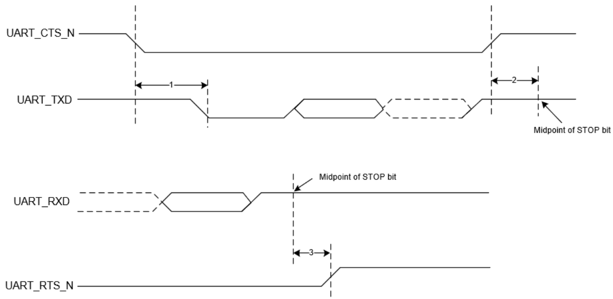
Figure 14. UART Timing
