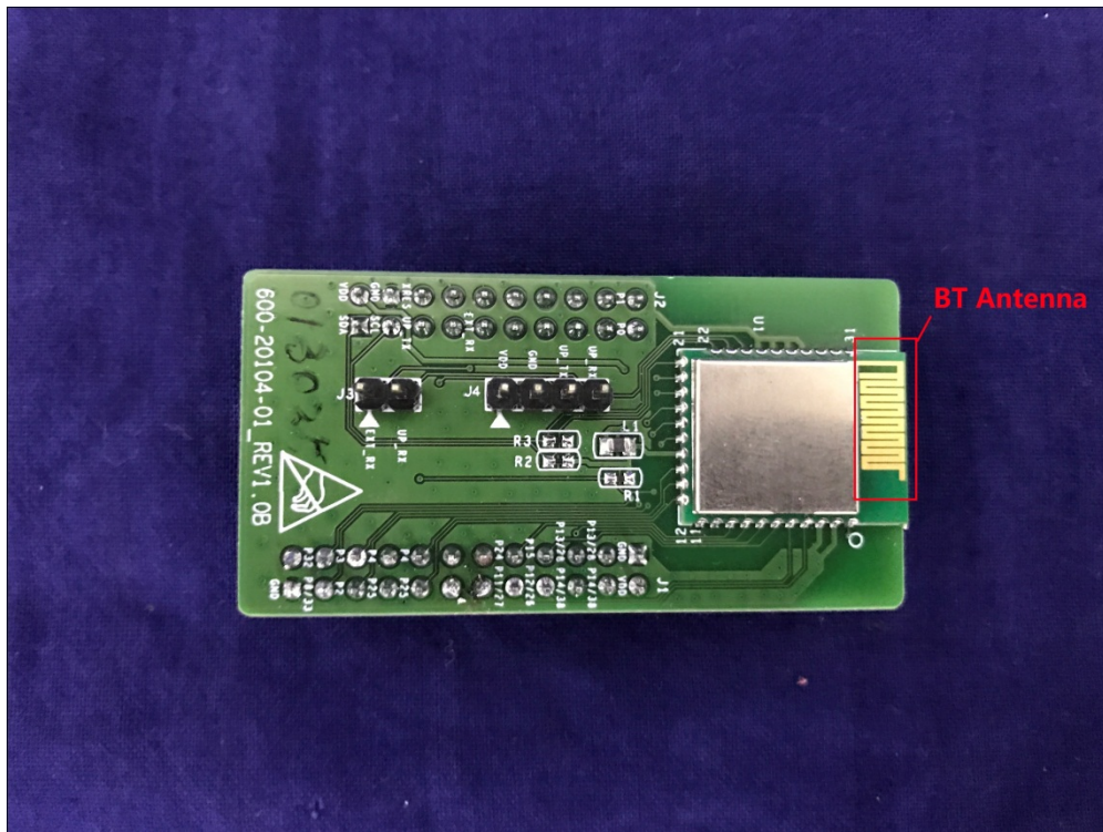
(2) EUT Photo(CYBLE-013025-00)
