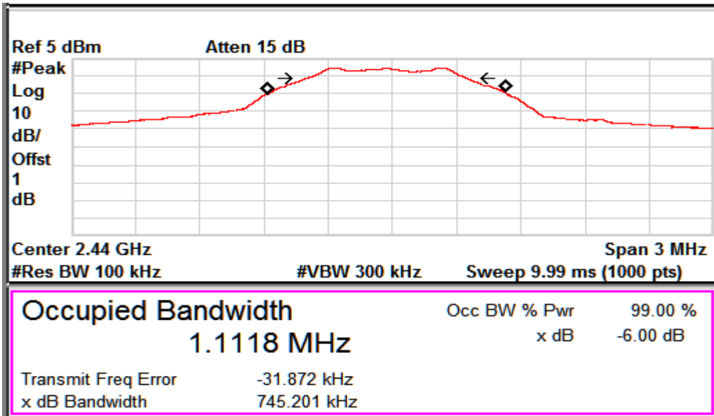
6dB BW and OBW: Channel frequency: 2440 MHz
