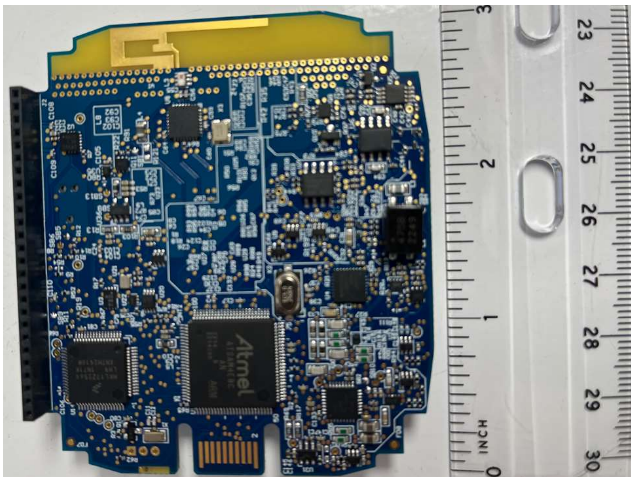
Pioneer G2MCU, Alog, RF PC Assembly Top
