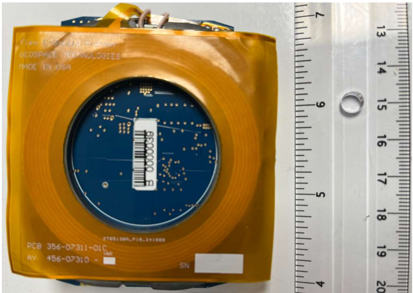
Pioneer WP, PS PC Assembly Bottom
