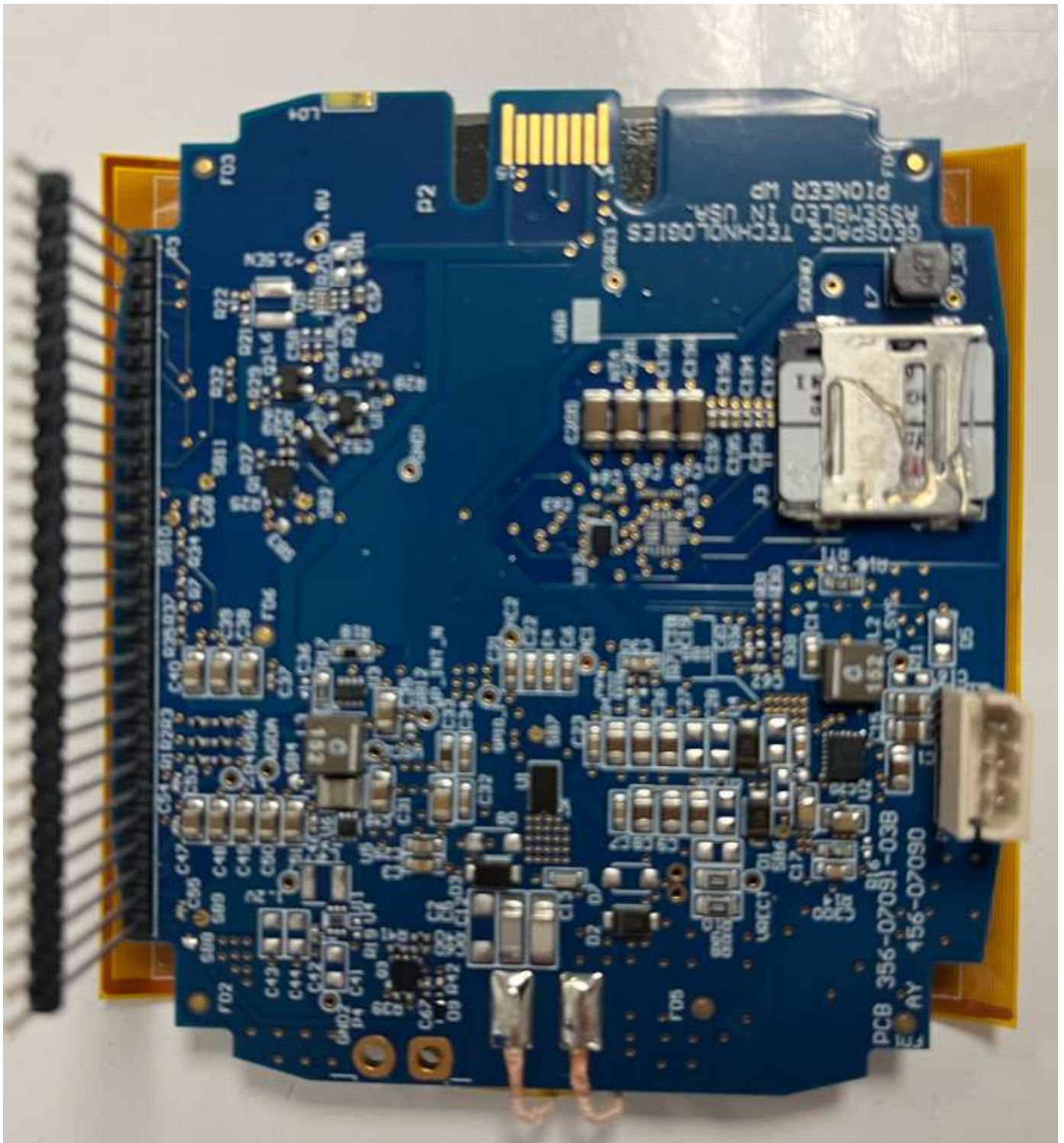
Pioneer WP, PS PC Assembly Top
