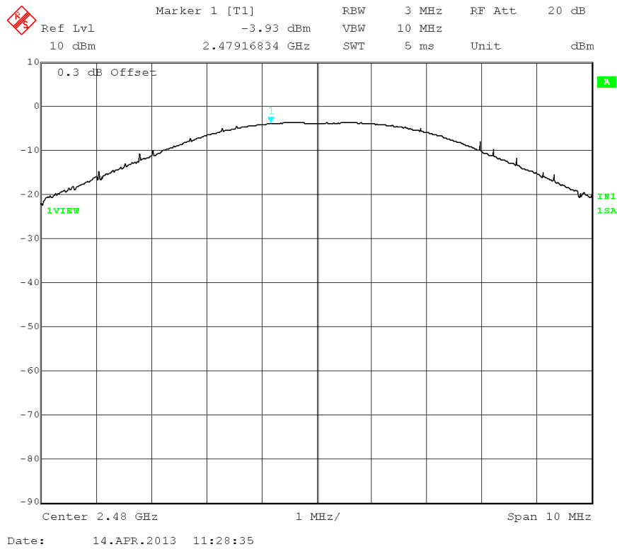
Output Power High Channel
