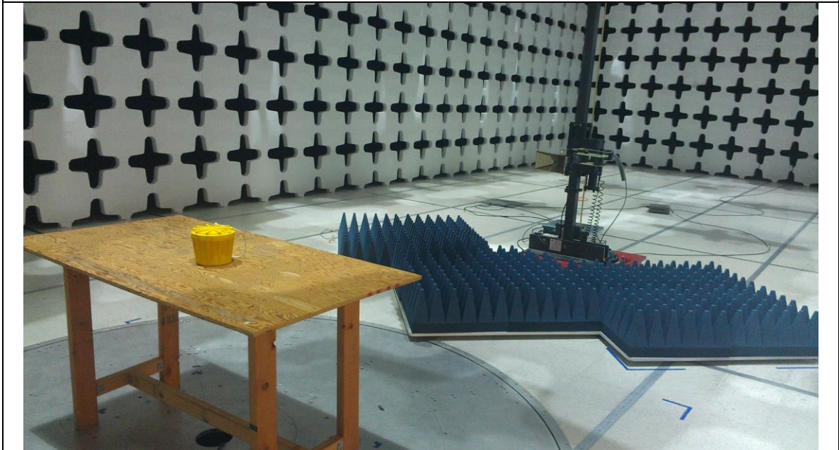
Radiated Emission Test Setup (above 1GHz) – Rear View
