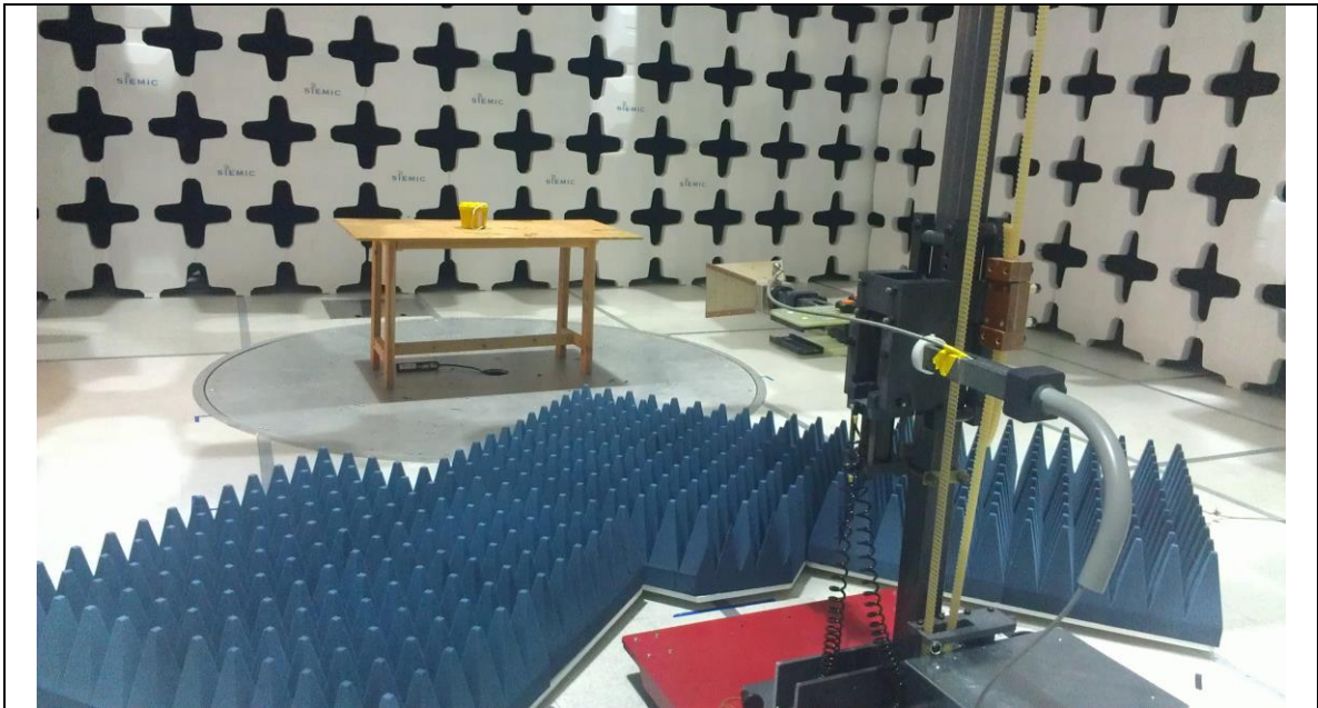
Radiated Emission Test Setup (above 1GHz) - Front View
