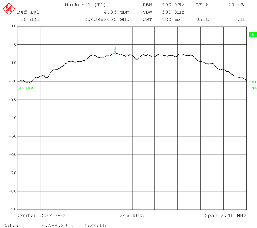
PSD Mid Channel
