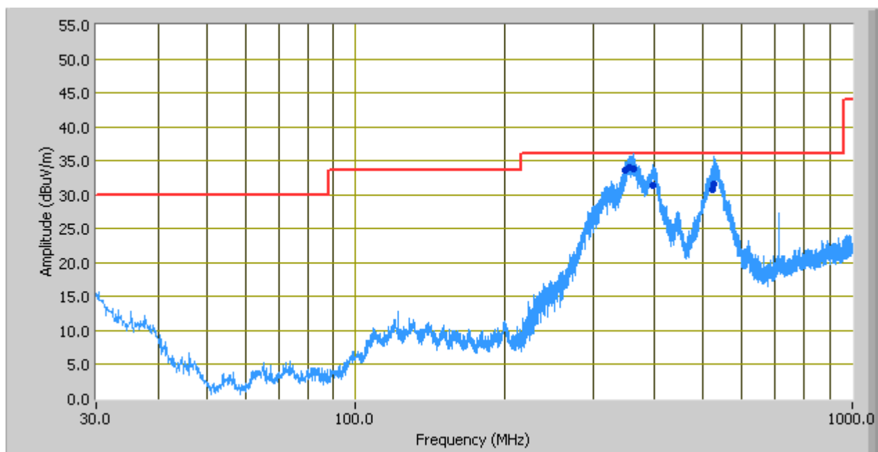
Radiated Emission Plot @ 10m
