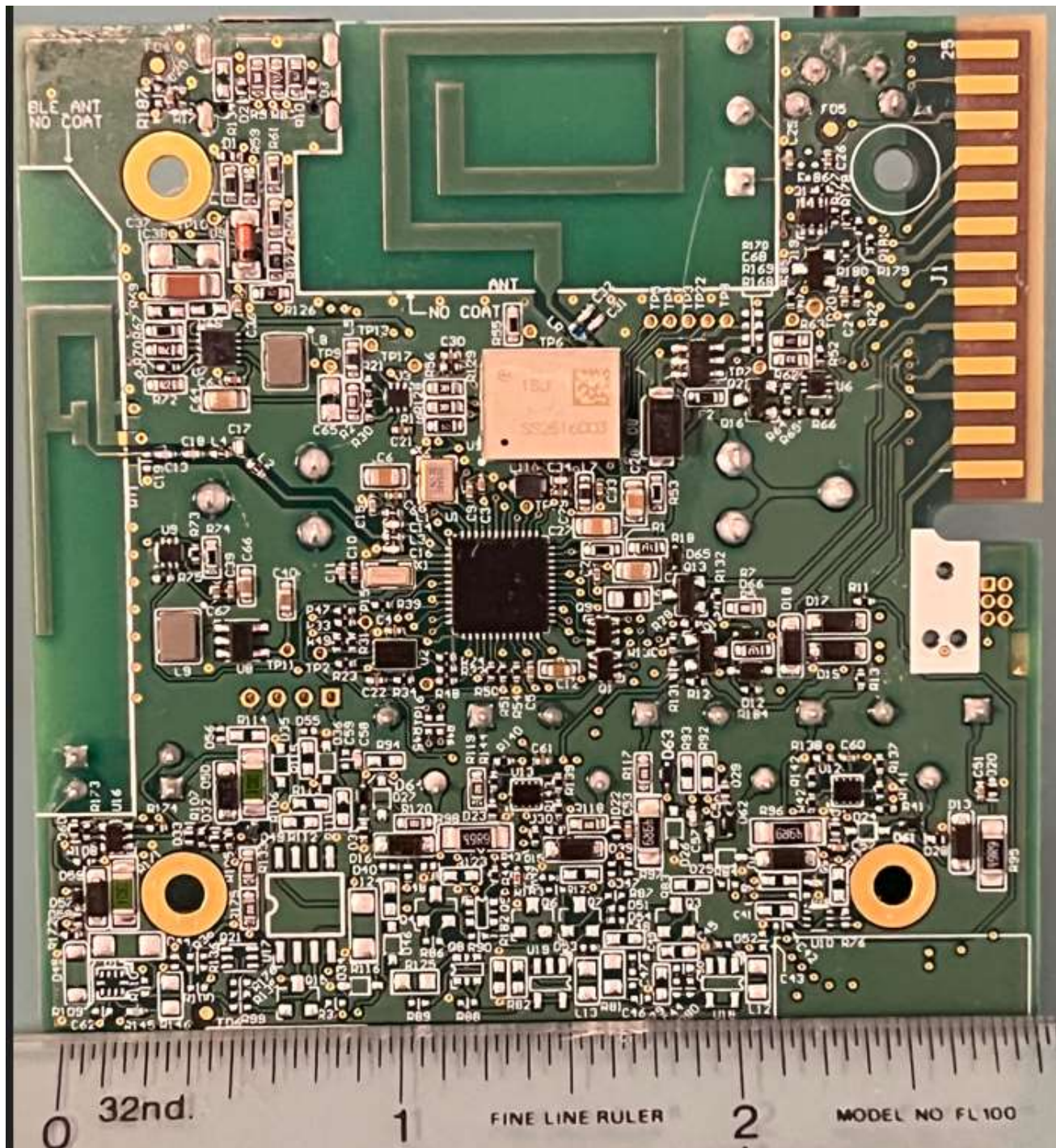
Bottom side of board showing BLE antenna to the left and LoRa antenna at the top
