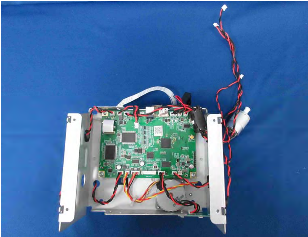
(38) EUT Photo
