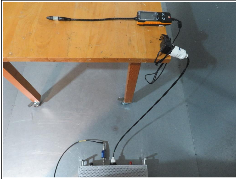
Setup EUT with AC/DC adapter (EGSTON)
